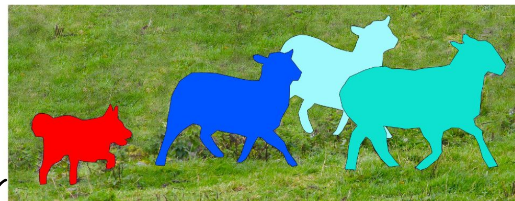
Instance Segmentation
