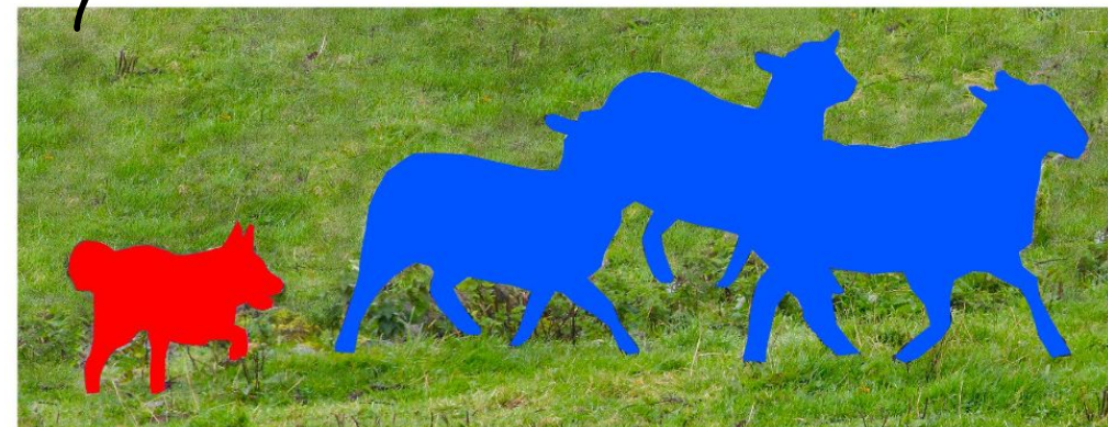
Semantic Segmentation
