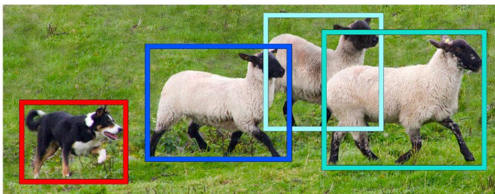
Object Detection
