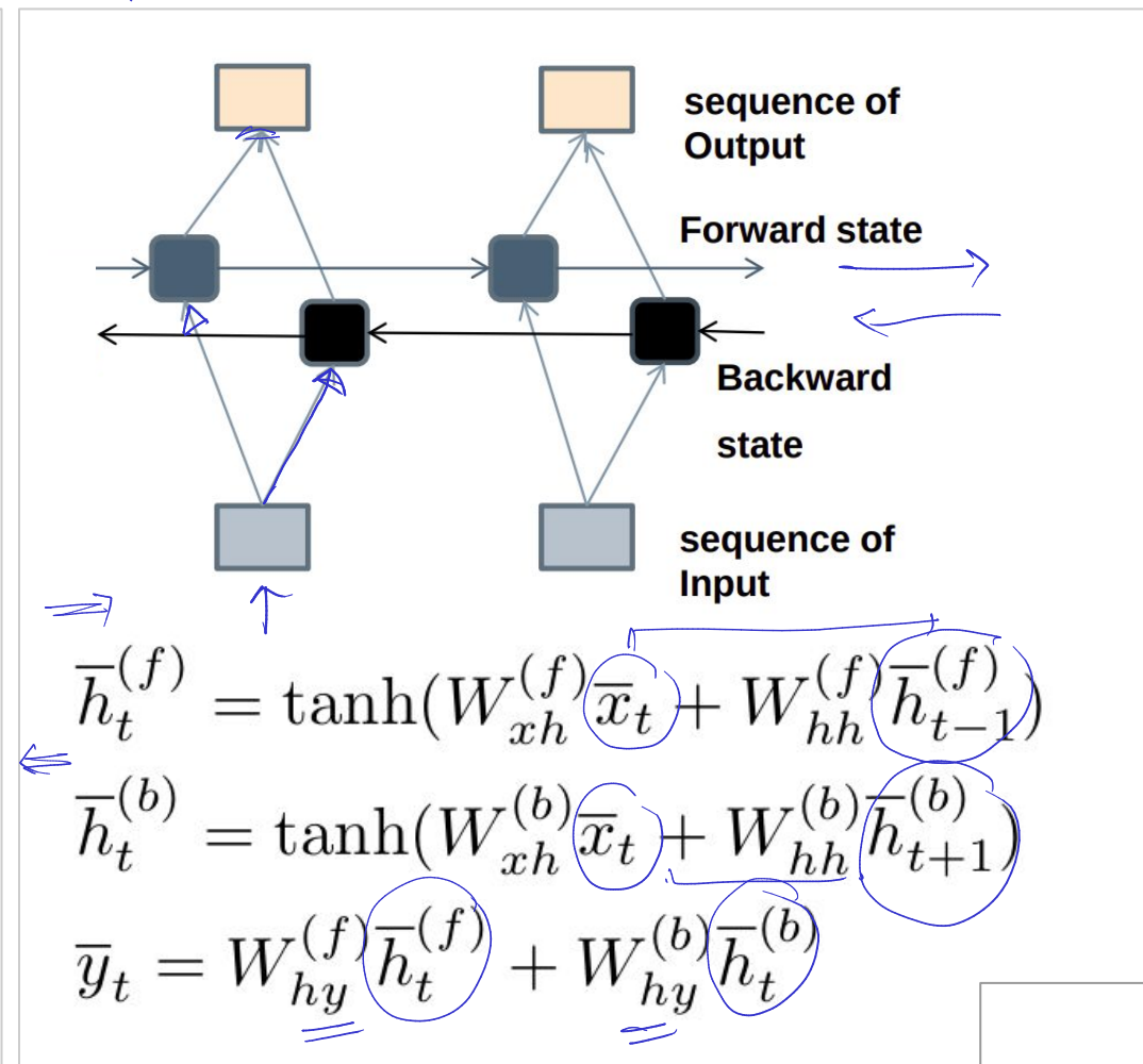
Bidirectional recurrent neural network
