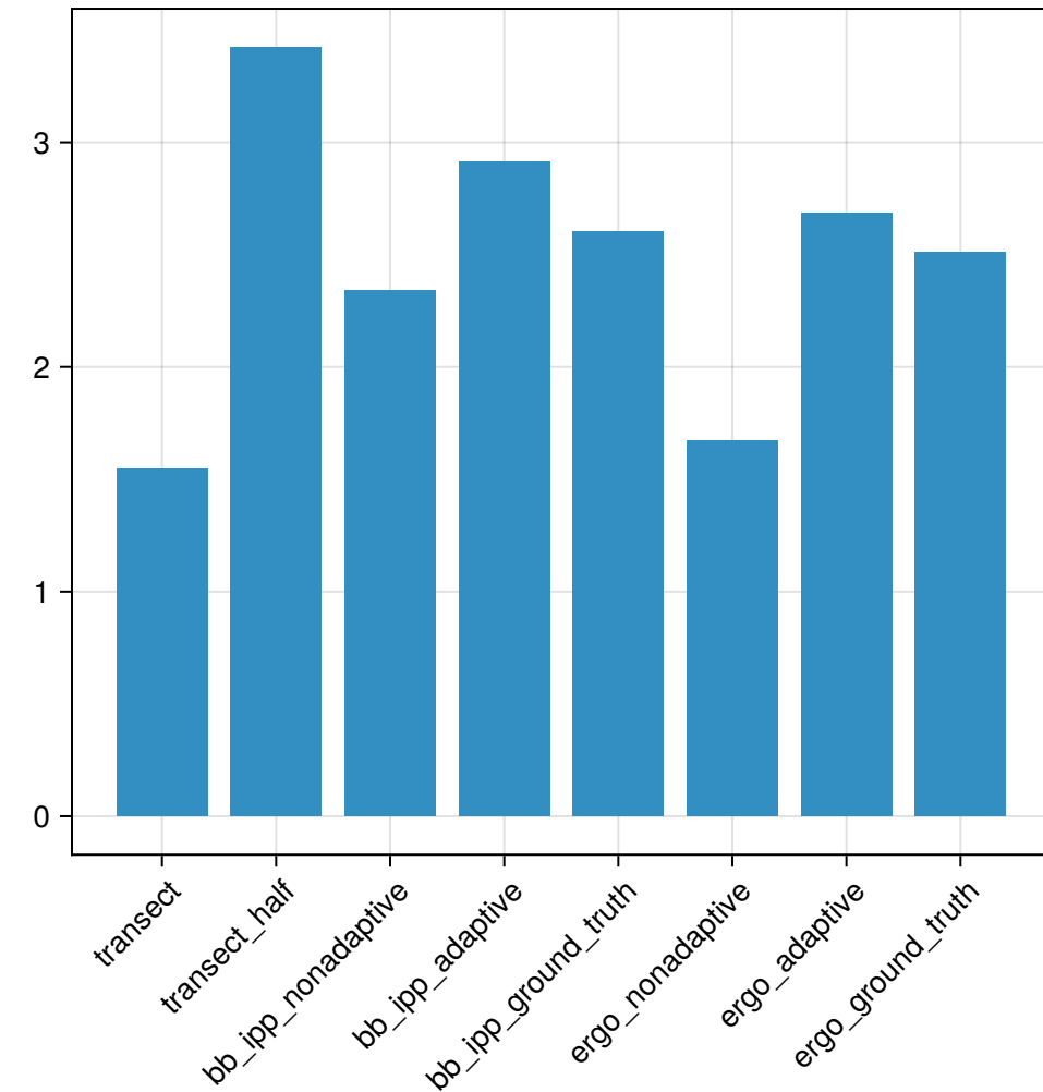
Global RMSE
