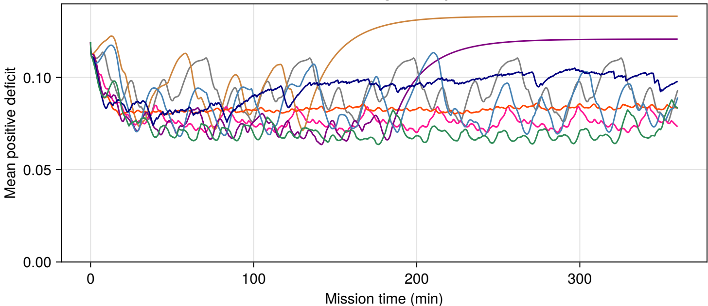
Ground-truth-target clarity deficit
