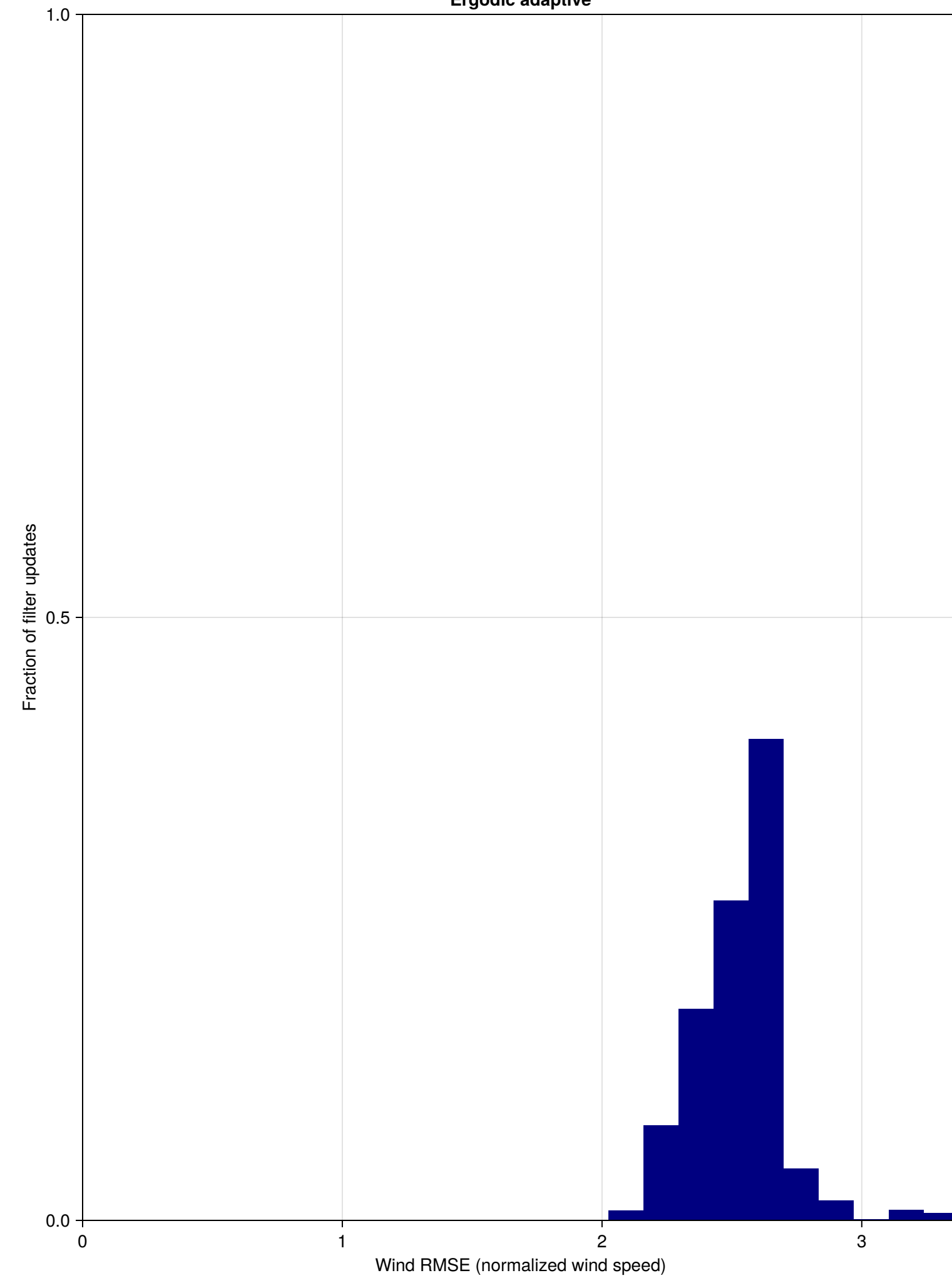
Wind RMSE distributions within each mission
