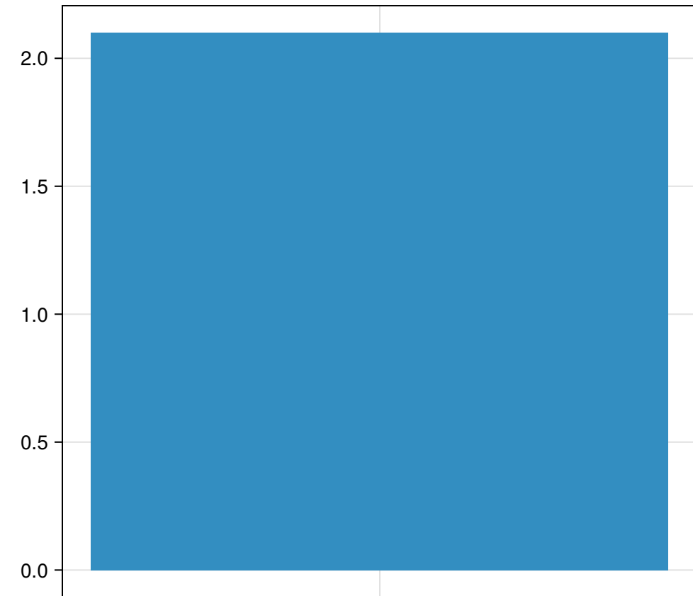
Global RMSE
