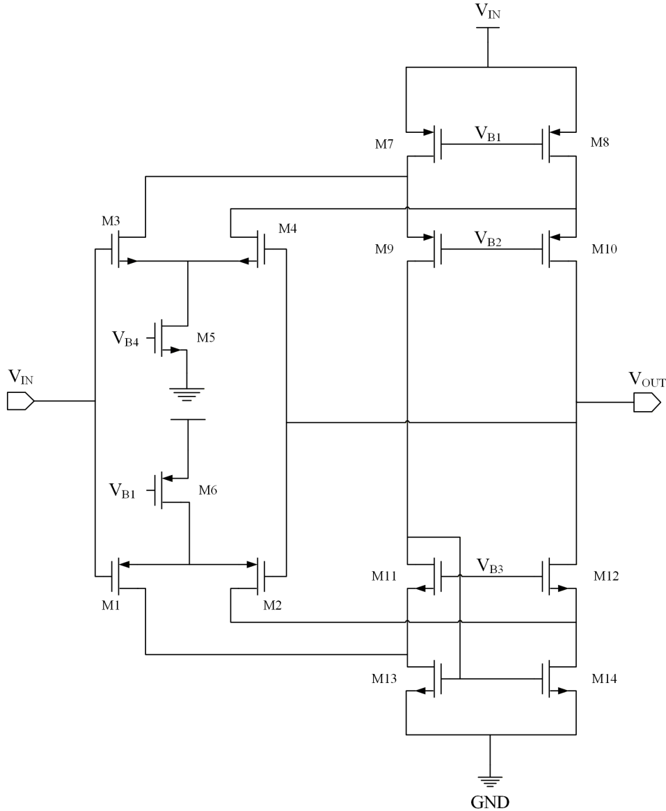
Figure 6 opa2 电路图
