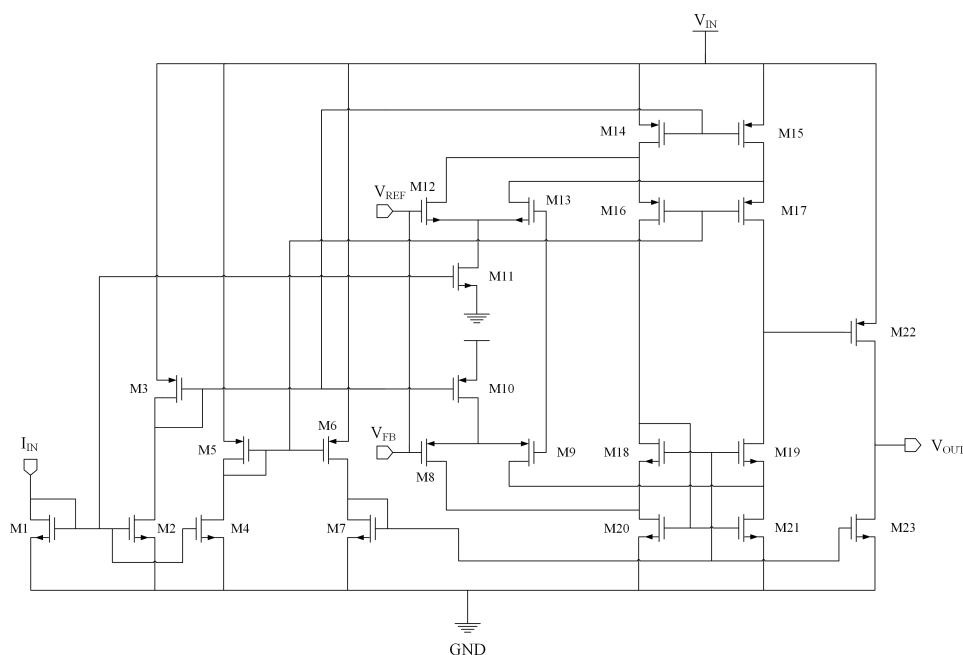
Figure 5 opa1 电路图
