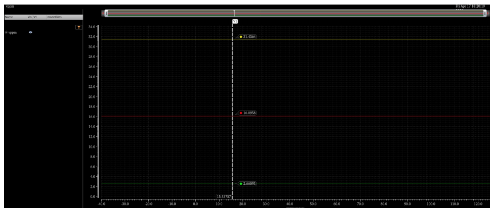
Figure 11 bandgap 输出温漂系数
