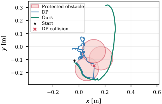
(a) Executed EEF trajectories (top view)
