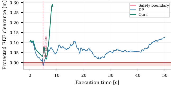
(b) Clearance during execution
