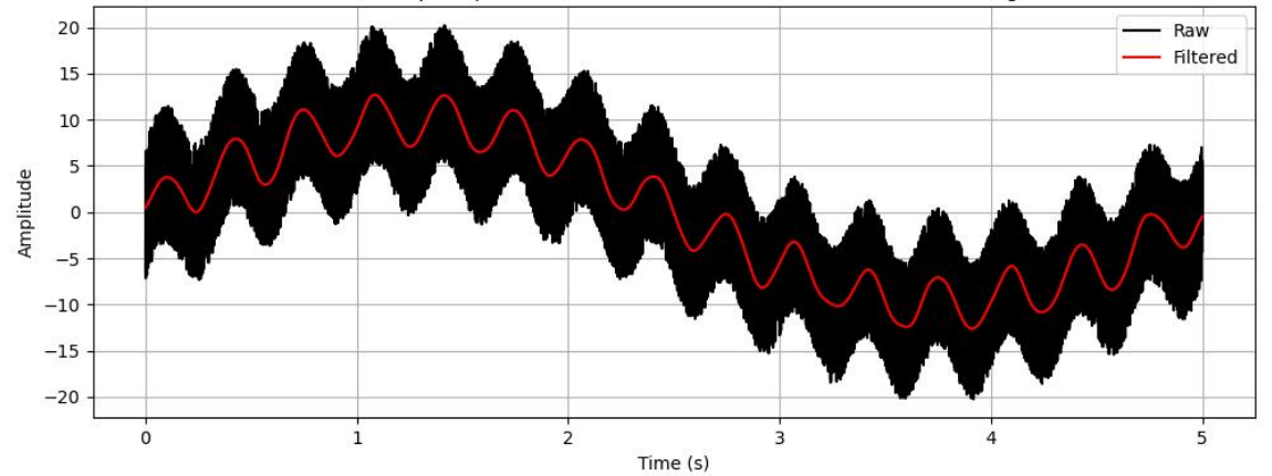
FIR Low-pass | Bandwidth=13.2, cutoff=4 Hz, window=Hamming
