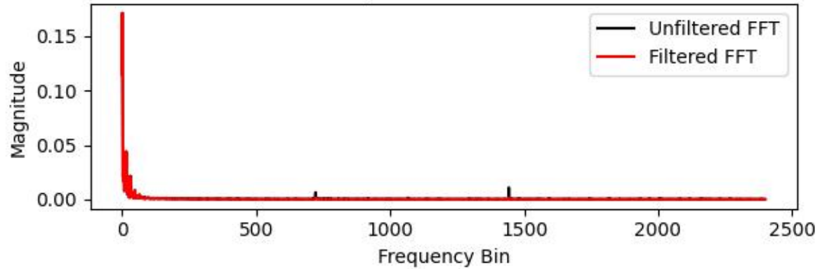
FFT Comparison (A=0.8, B=0.2)
