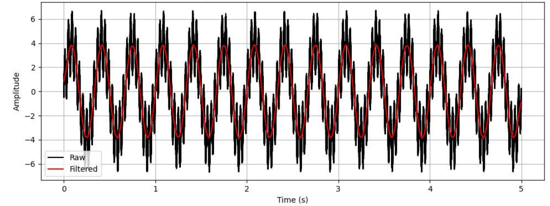
FIR Low-pass | Bandwidth=40.0, cutoff=5 Hz, window=Hamming
