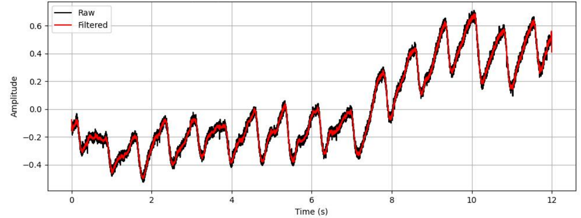
FIR Low-pass | Bandwidth=20.0, cutoff=30 Hz, window=Hamming
