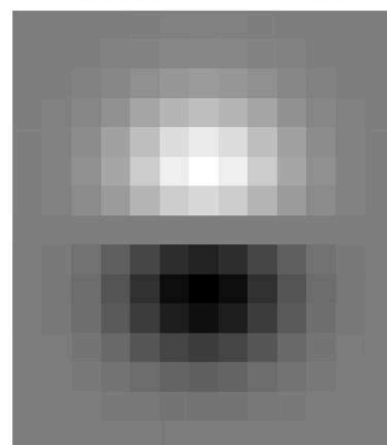
Derivative-of-Gaussian D_y
