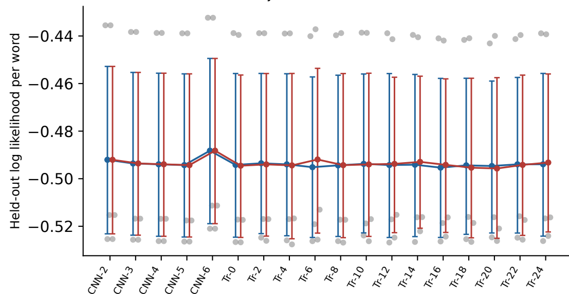
Feature space
