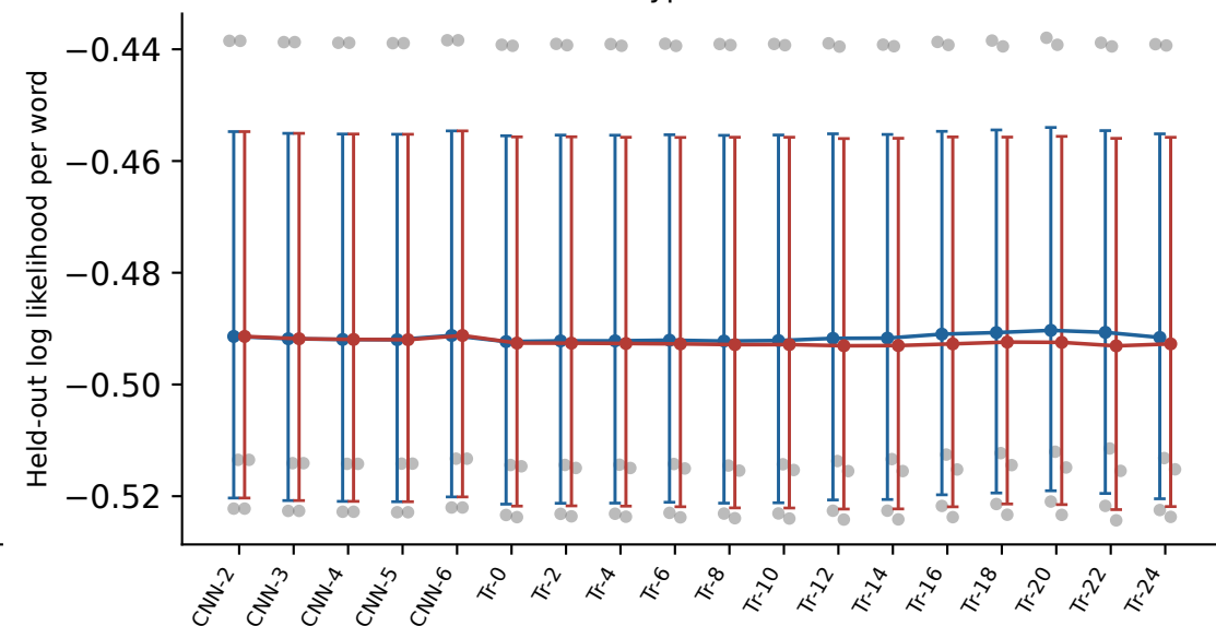
Feature space
