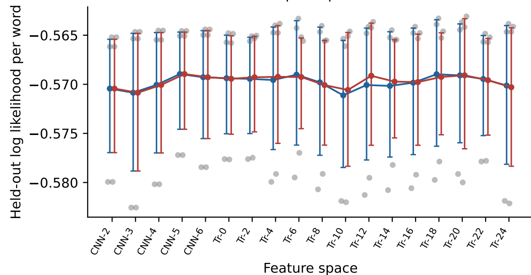
Adjacent frames: word 168 participants
