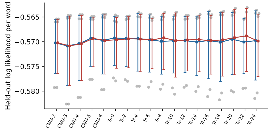
Adjacent frames: word 168 participants
