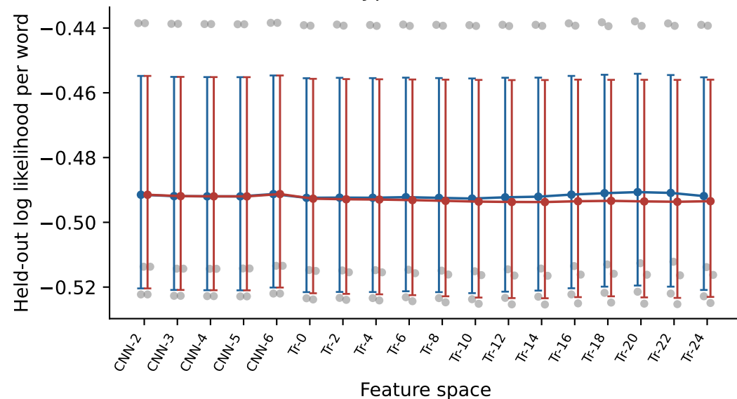
Adjacent frames: phoneme
