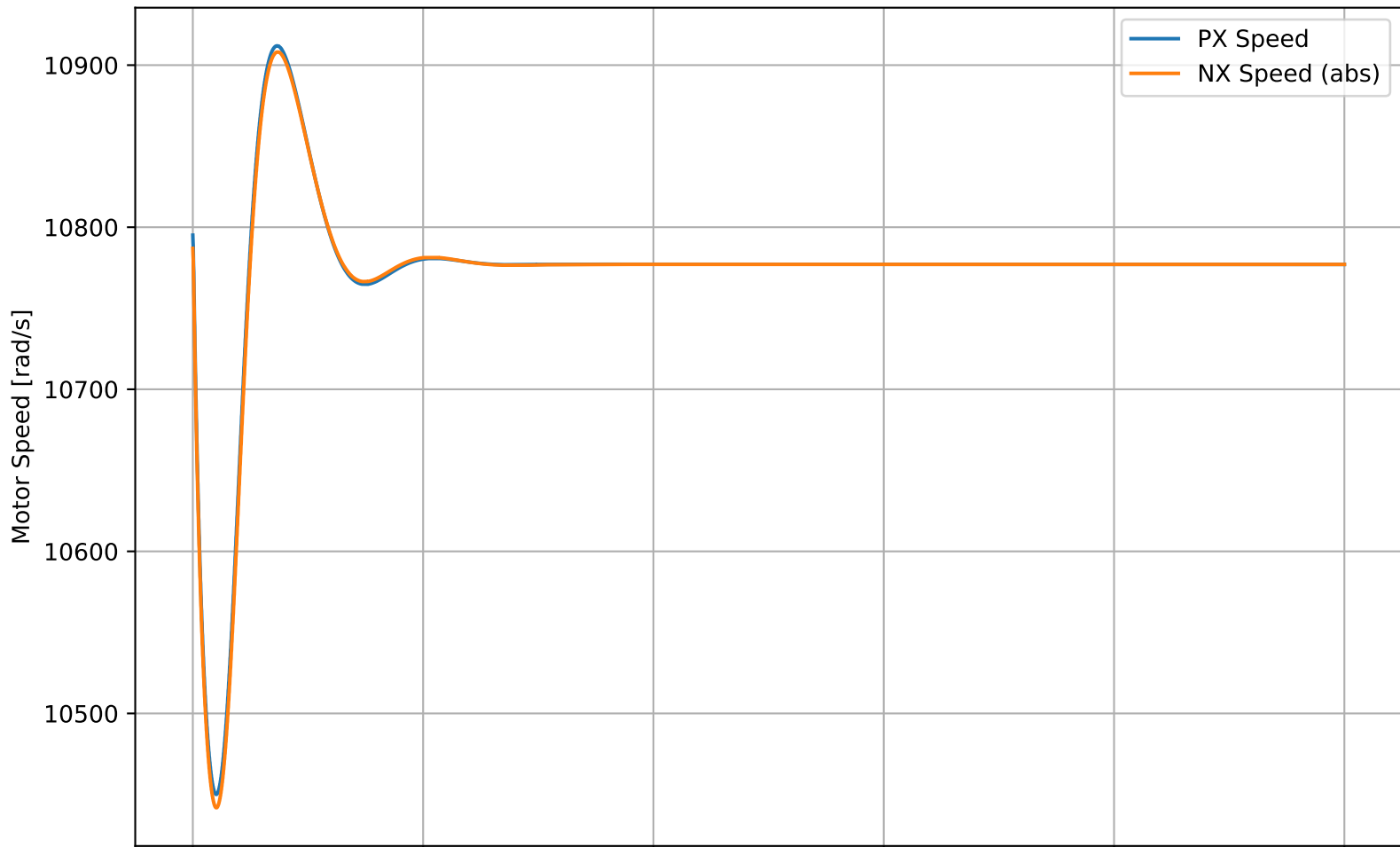
Motor Dynamics (Speeds & Accels)
