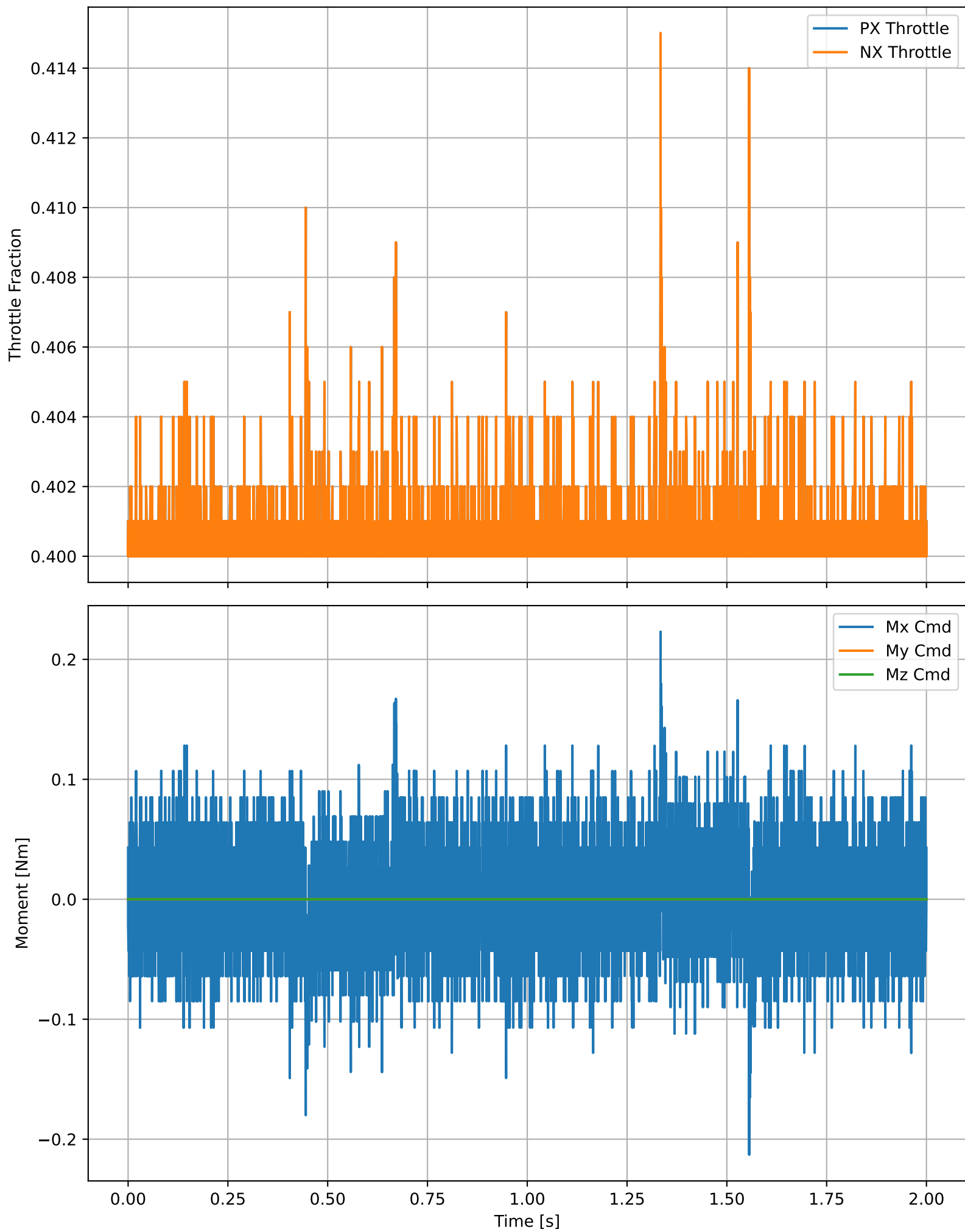
Control Efforts
