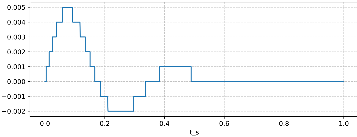
phidot_px_radps
