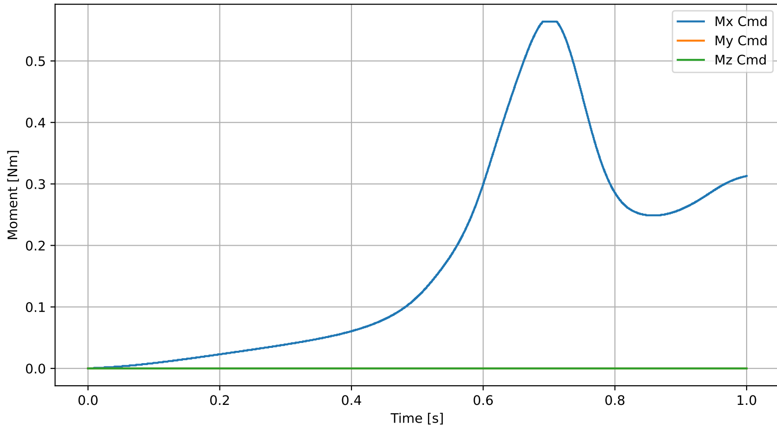
Commanded Control Moments
