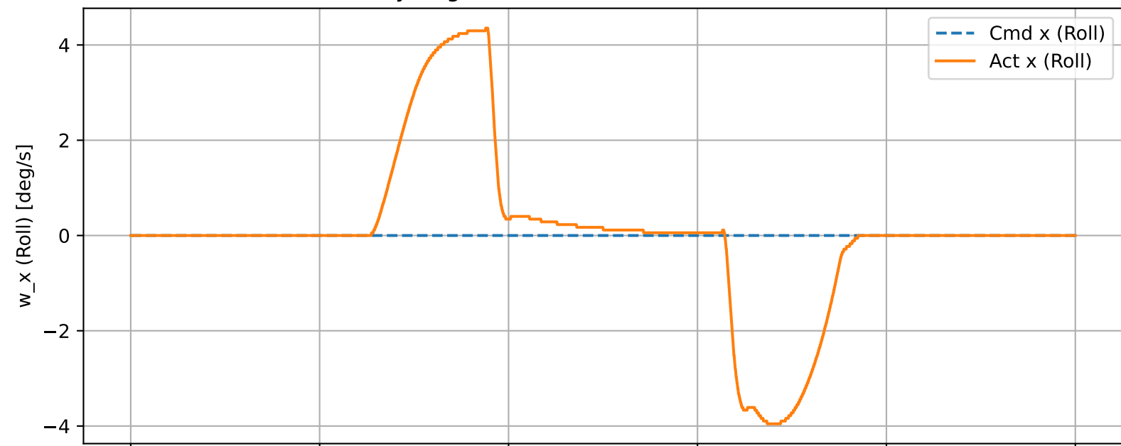
Body Angular Rates: Commanded vs. Actual
