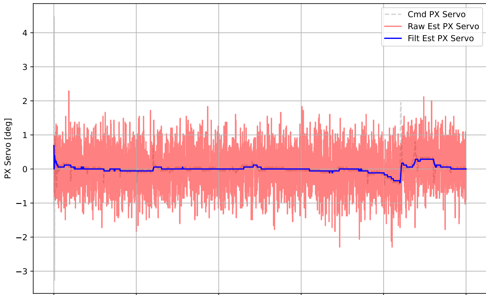
Servo Estimates: Raw vs. Filtered
