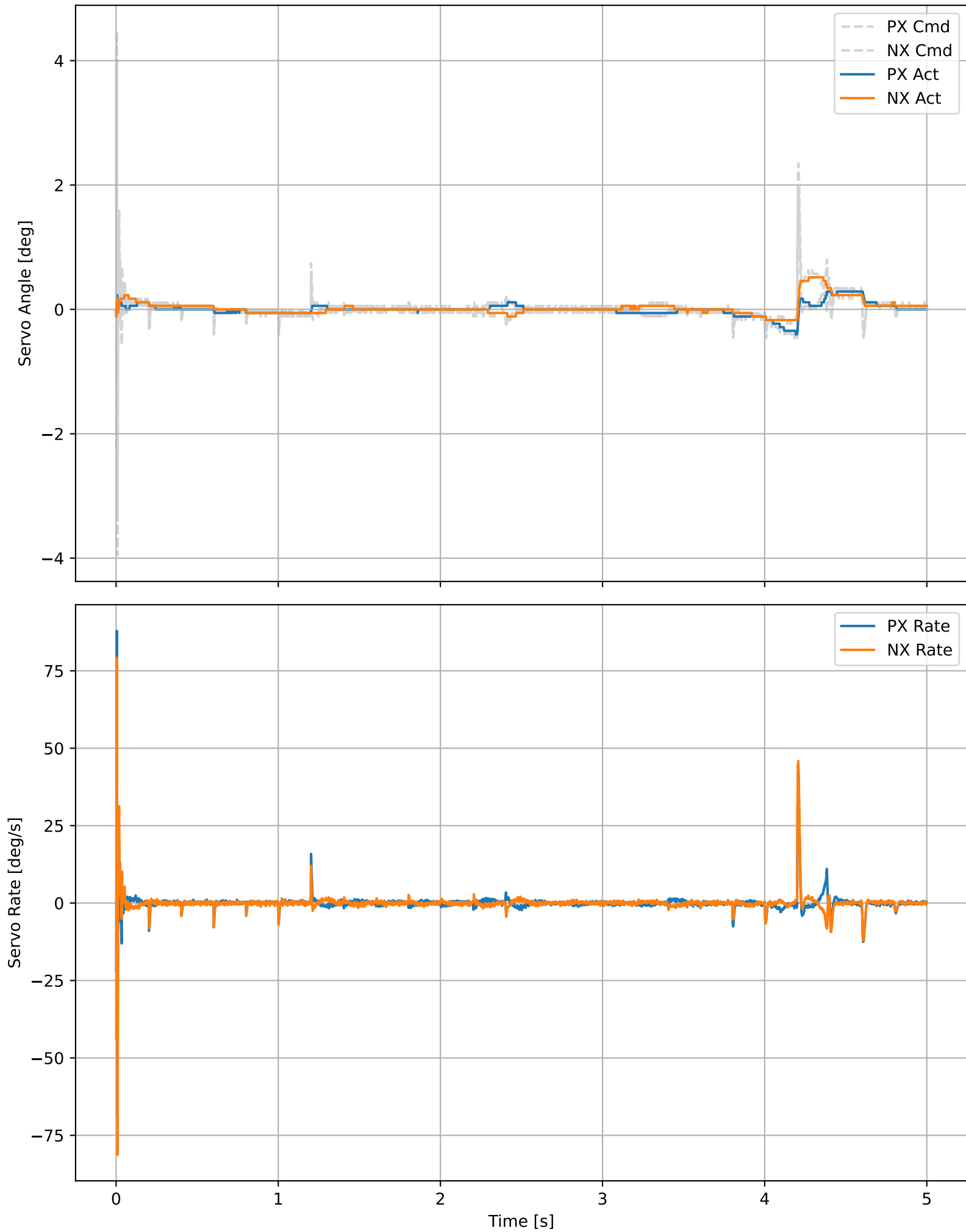
Servo Dynamics (Angles & Rates)
