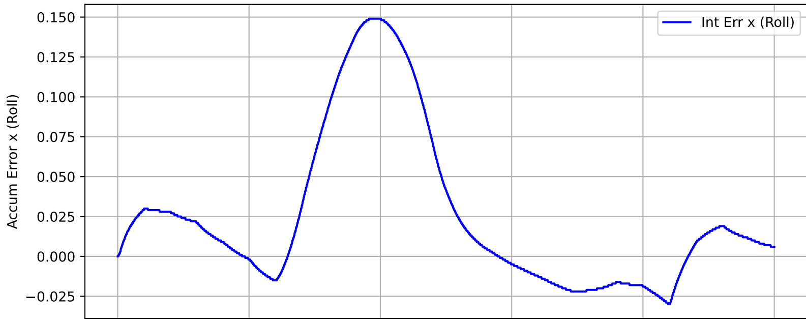
GNC Integrator State (Accumulated Error)
