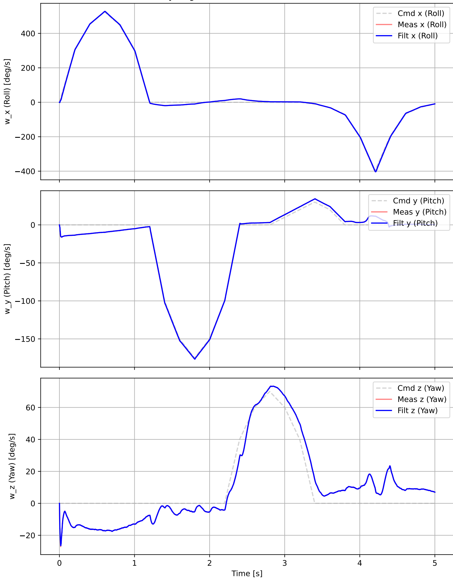
Body Angular Rates: Cmd vs. Meas vs. Filt
