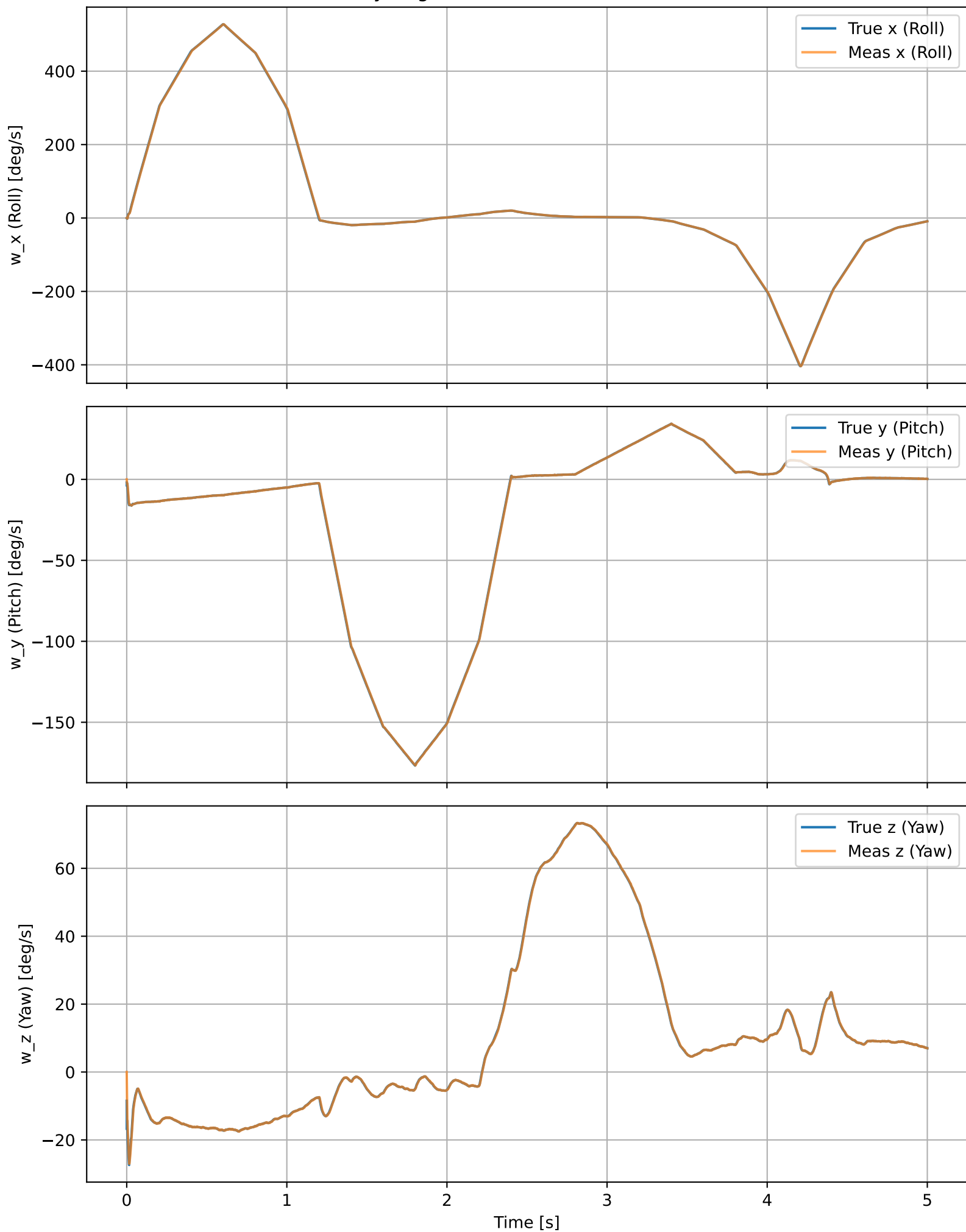
Body Angular Rates: True vs. Measured
