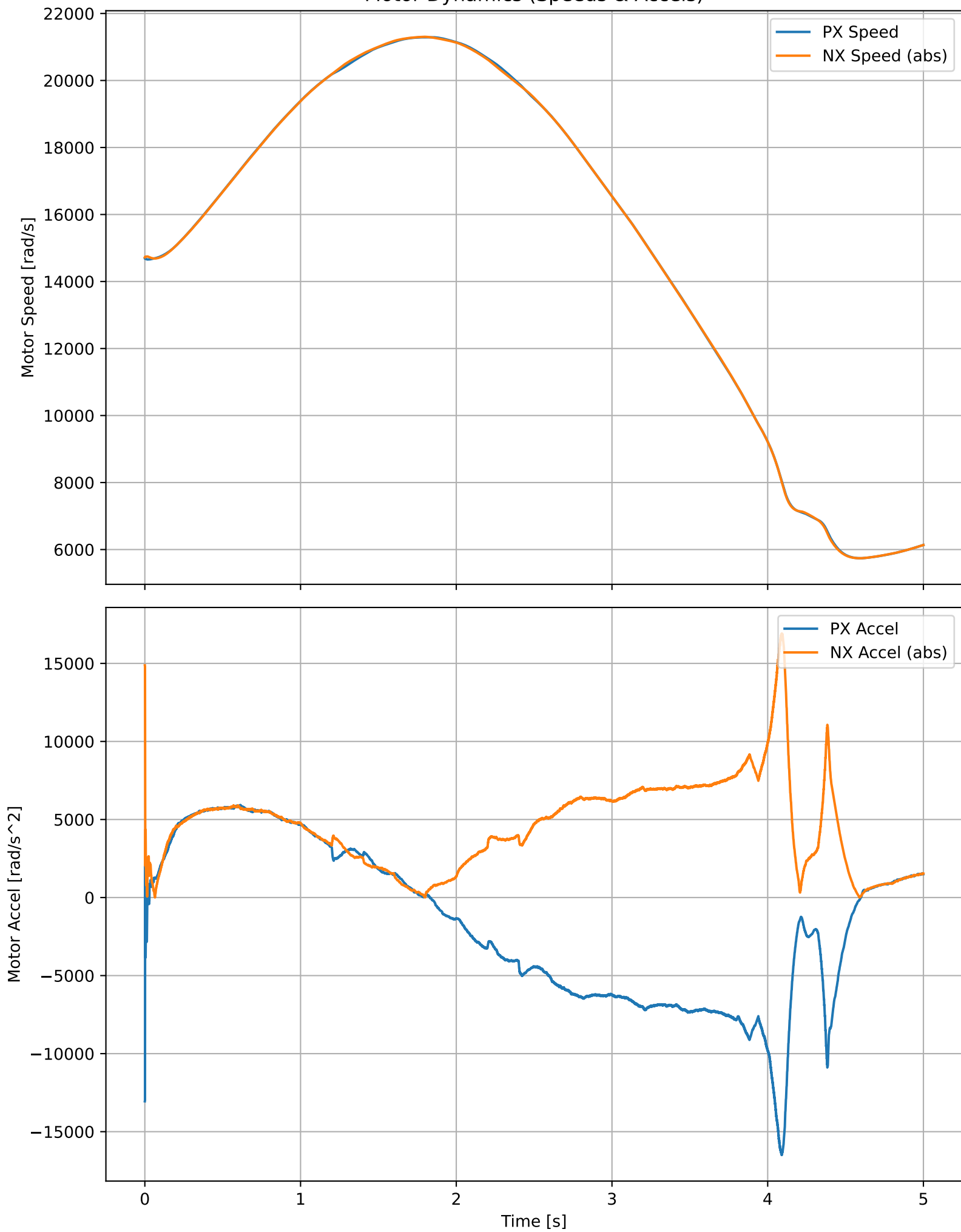
Motor Dynamics (Speeds & Accels)
