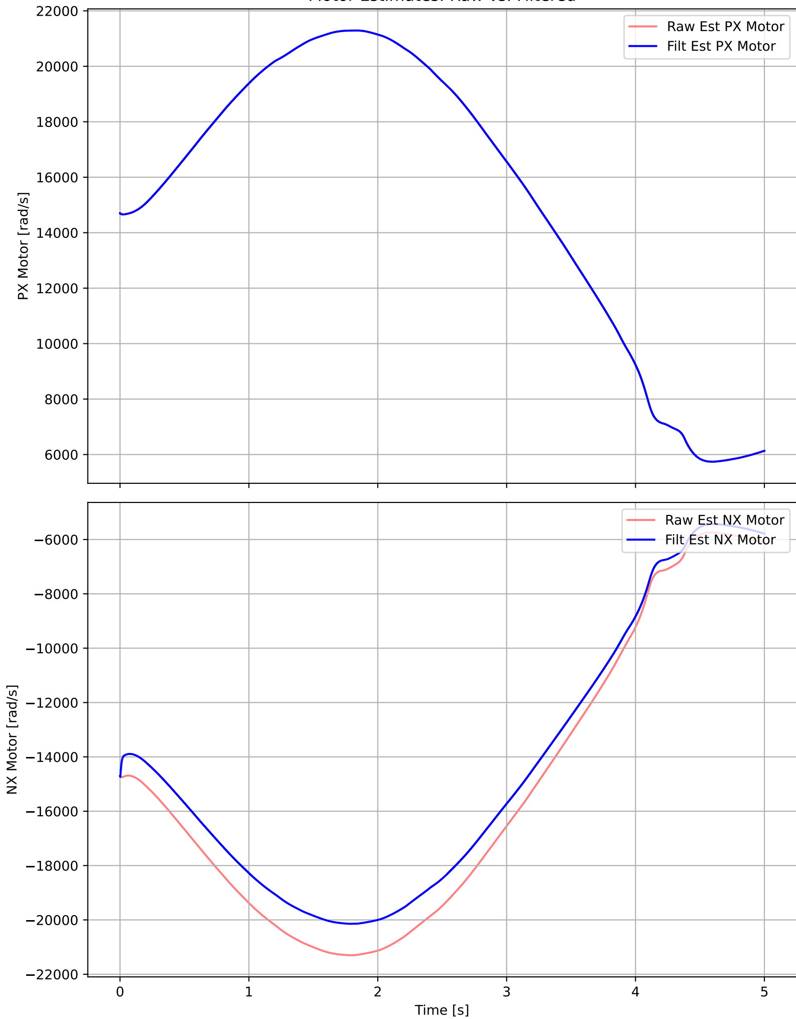
Motor Estimates: Raw vs. Filtered
