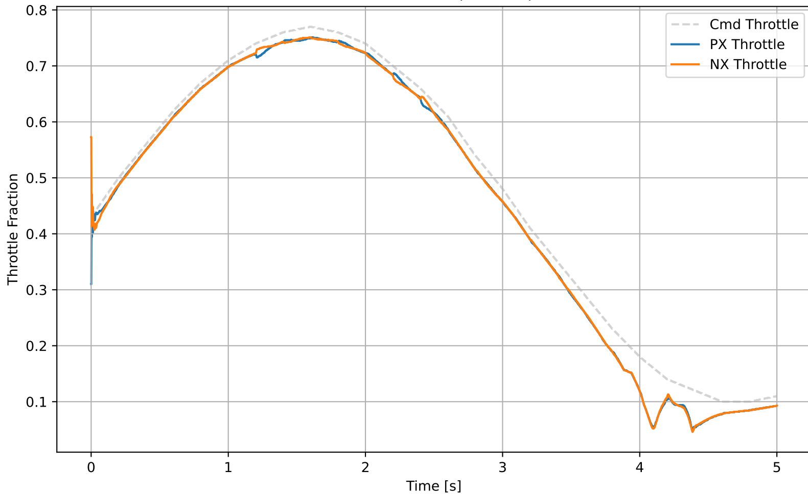
Control Efforts (Throttle)
