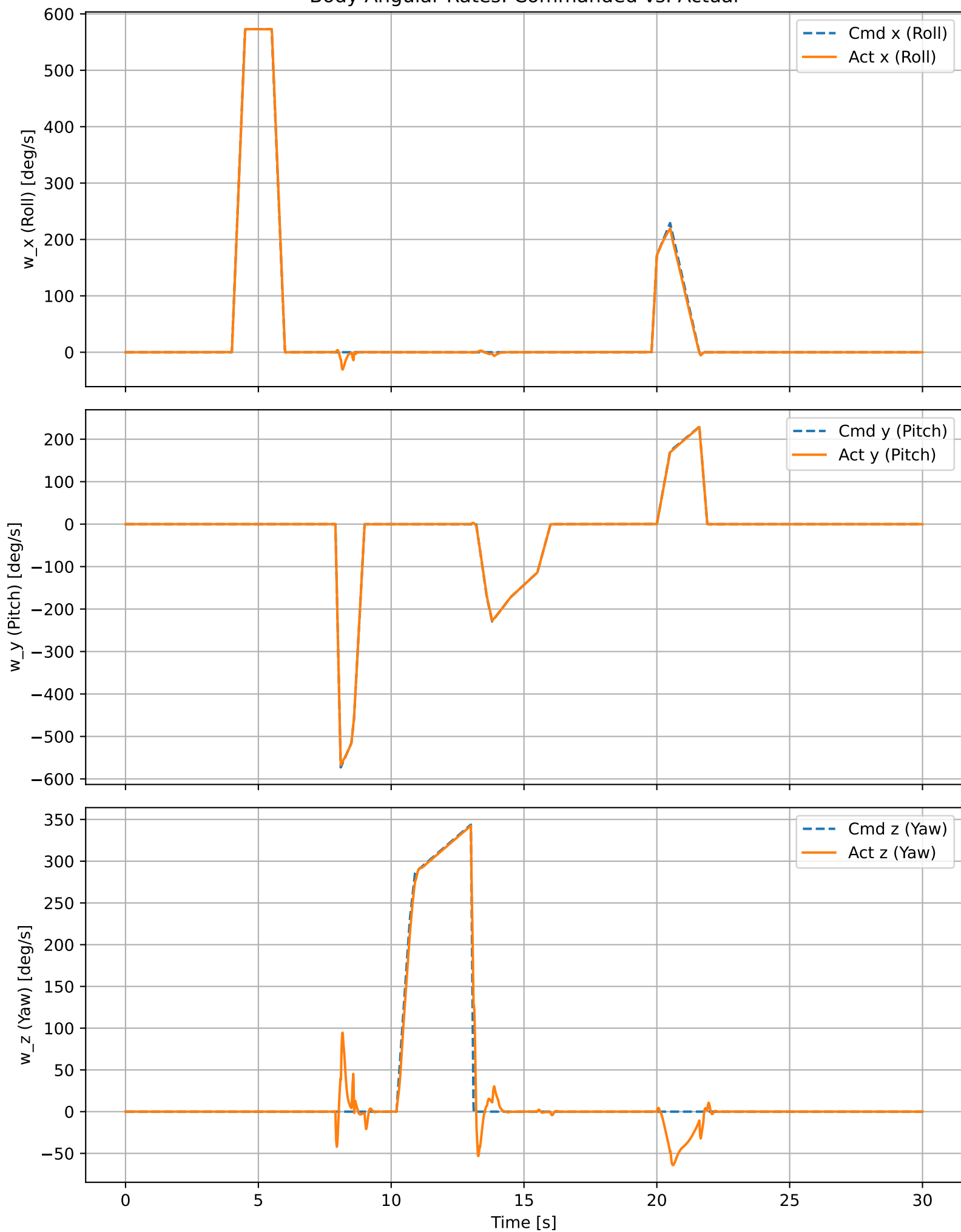
Body Angular Rates: Commanded vs. Actual
