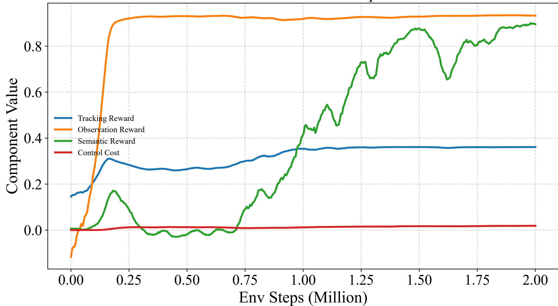
STG-MAPPO Reward Components
