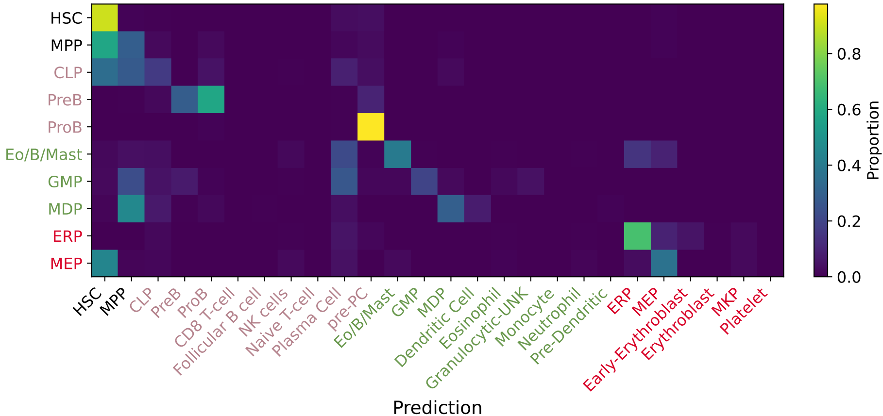
Confusion Matrix
