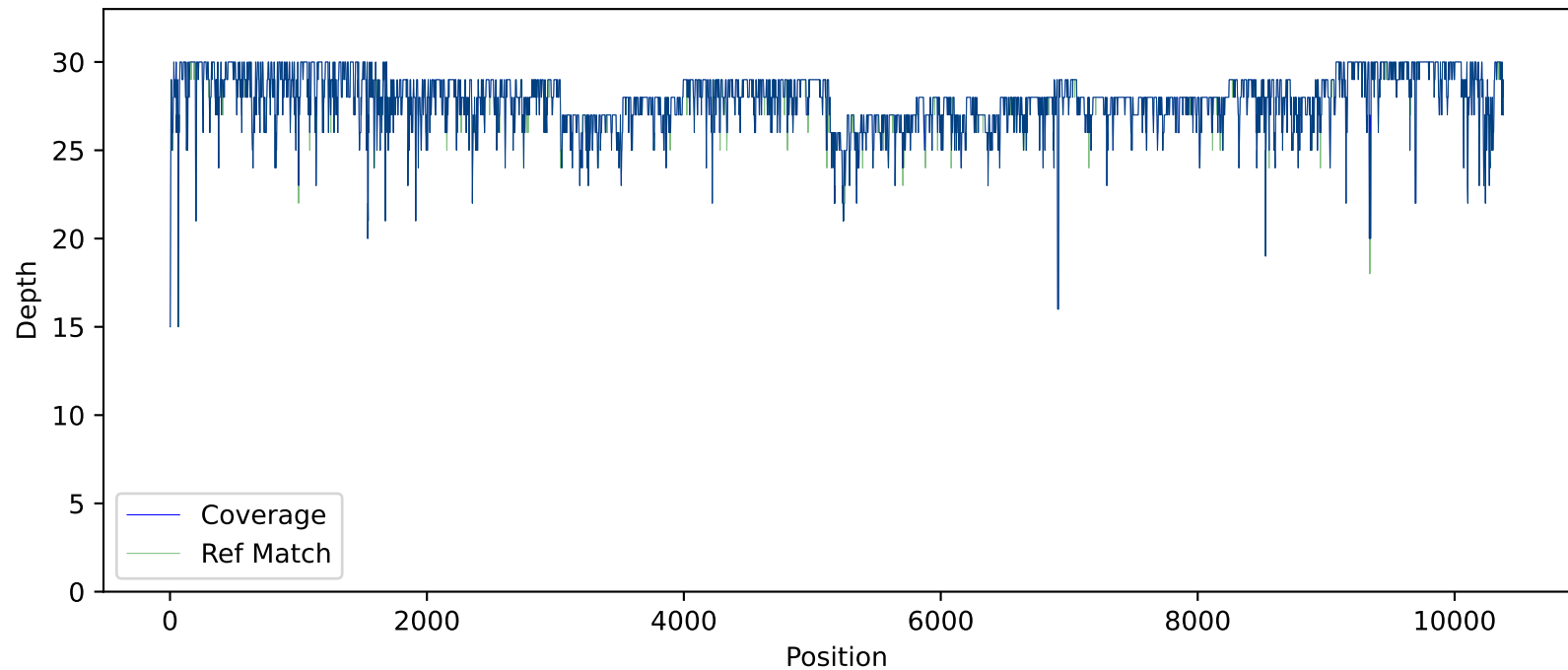
Coverage Plot for cole1-group-C3
