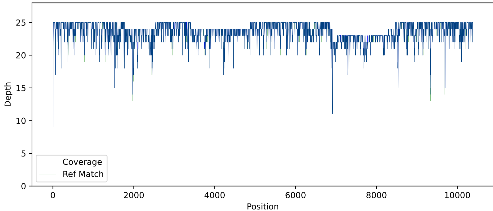
Coverage Plot for cole1-group-F1
