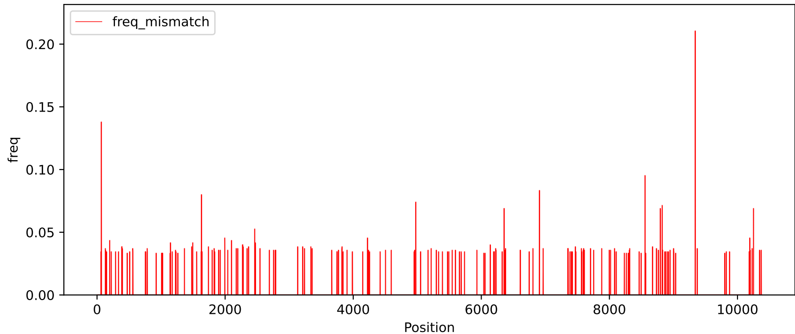
Substitution Plot for cole1-group-C5
