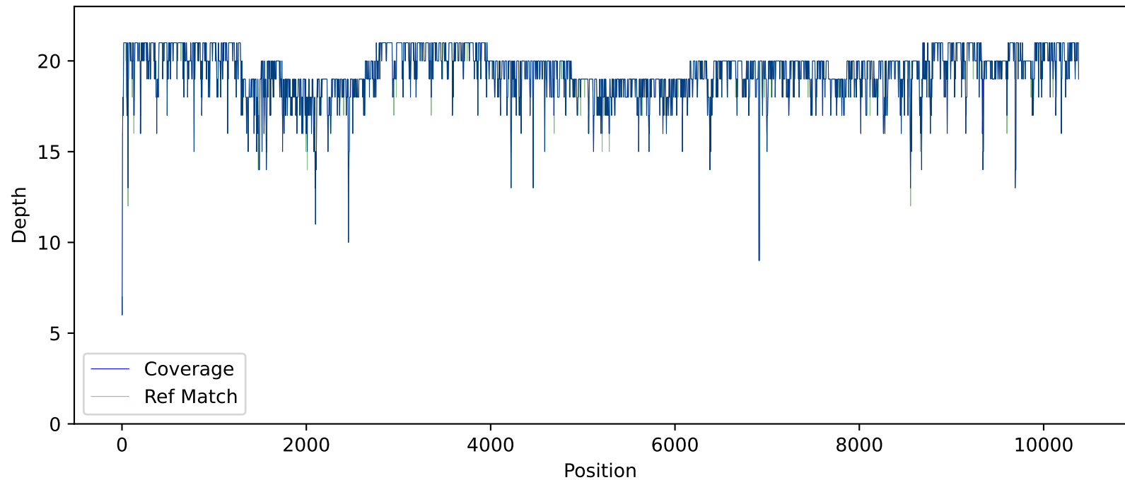
Coverage Plot for cole1-group-D5
