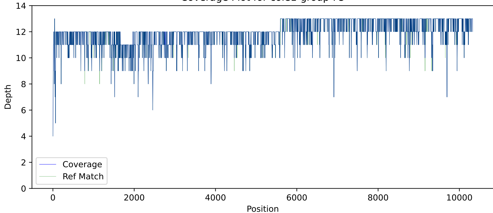
Coverage Plot for cole1-group-F5
