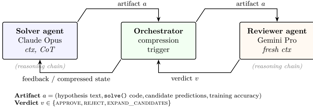
Figure 1: System pipeline. The solver (Claude Opus) and reviewer (Gemini 3.1 Pro, fresh context per puzzle) exchange only artifacts; reasoning chains stay local to each agent. The orchestrator routes artifacts and triggers compression (on a context-size threshold or on REJECT).
