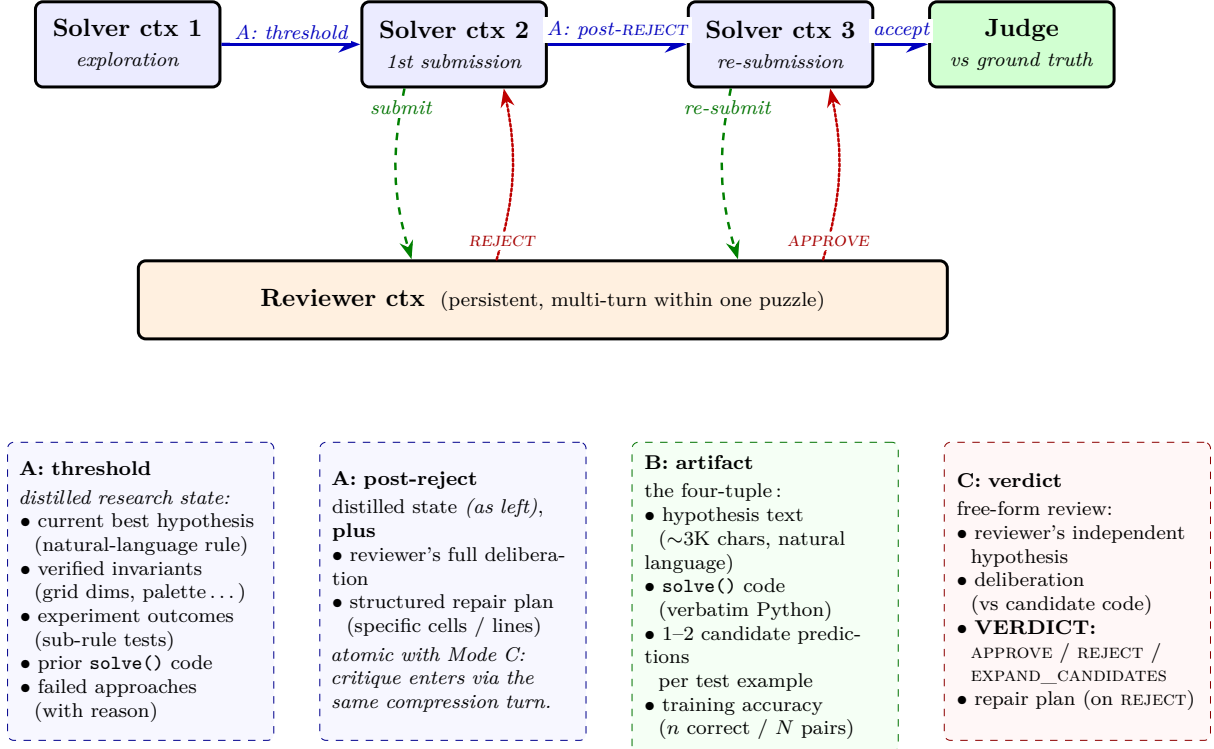
Figure 2: The three modes of Inter-Context Artifact Exchange (ICAE), traced through a representative two-cycle solve. Each top-row blue box is a context-bounded model instance of the solver; the solver’s context is reset at the compression threshold \tau (Solver ctx 1→2, Mode A solid) and again on reviewer REJECT (Solver ctx 2→3, Mode A atomic with the rejection). The bottom orange box is the reviewer’s persistent multi-turn context, which receives solver artifacts ( Mode B dashed) and returns verdicts to the submitting solver instance ( Mode C dotted). The dashed annotation boxes list the verbatim contents of each handover. The rightmost Judge node is the external ARC-AGI-2 grader against ground-truth test outputs; it is not part of Athanor and runs only after the reviewer issues APPROVE. There is no Mode D: reviewer output is bounded and never reaches the threshold \tau , so reviewer-to-reviewer self-handover is never required.
