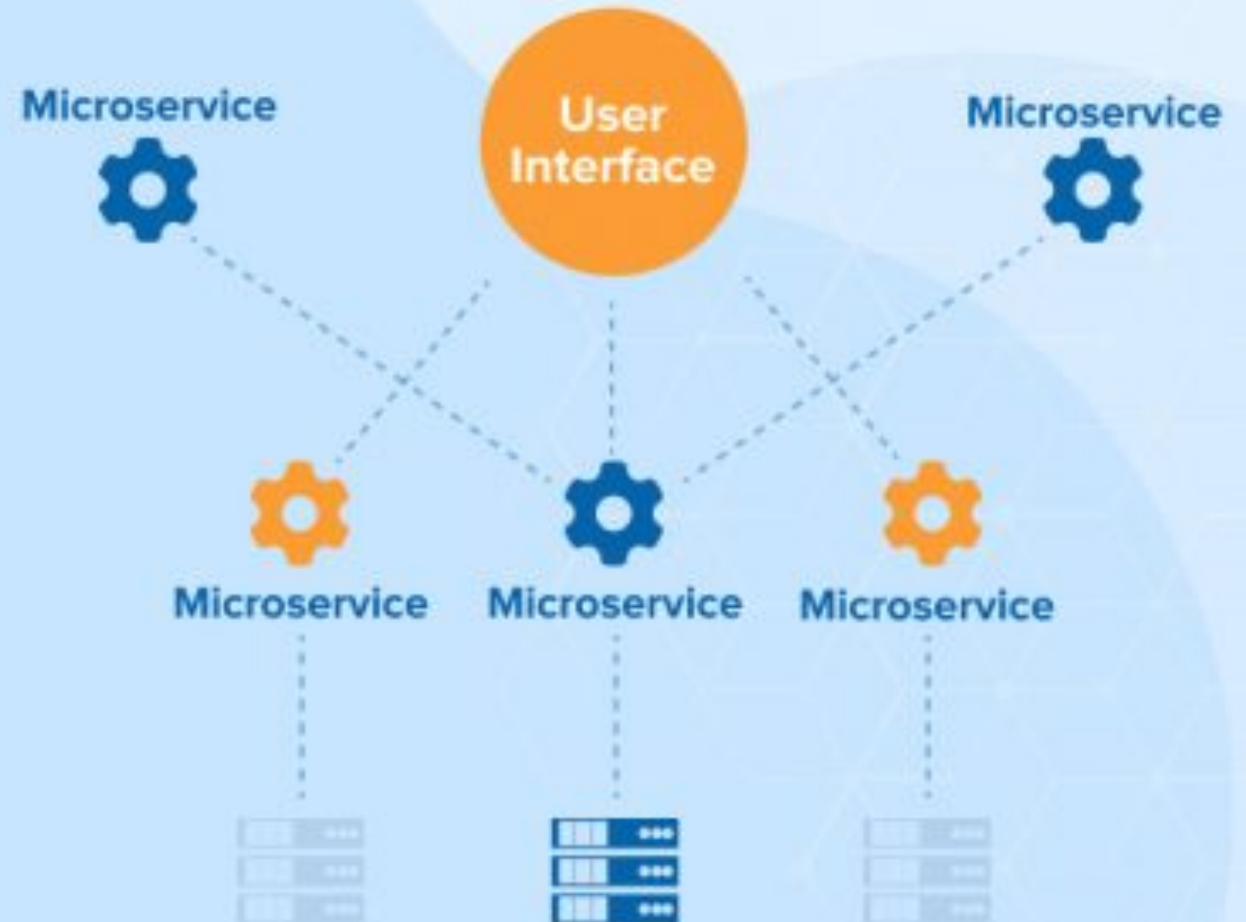
Microservices Architecture
