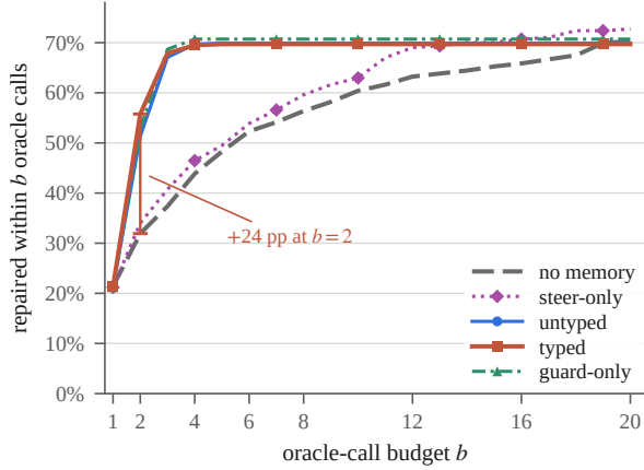
Fig. 1. The pre-specified primary metric: repair rate at a matched oracle-call budget b , five arms, 495 main and 297 ablation cells. Memory saturates by b=4 ; no memory needs b=20 for the same rate. STEER-ONLY tracks no memory, which is Section VII-C’s finding in one line.
