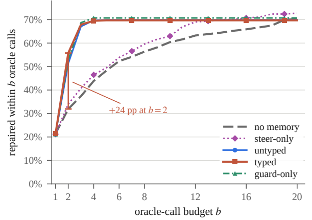
Fig. 1. The pre-specified primary metric: repair rate at a matched oracle-call budget b , five arms, 495 main and 297 ablation cells. Memory saturates by b=4 ; no memory needs b=20 for the same rate. STEER-ONLY tracks no memory, which is Section VII-C’s finding in one line.
