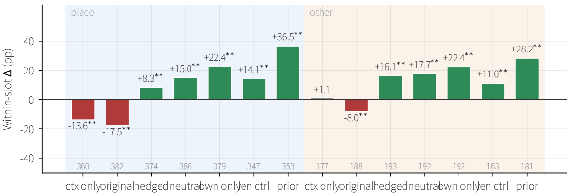
Qwen2.5-VL (3B / 7B)
