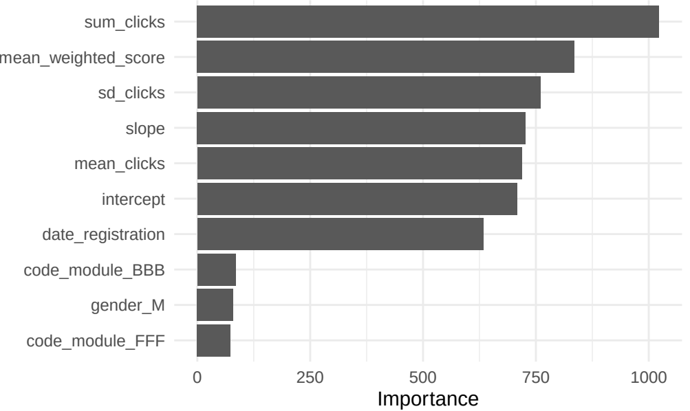
Top 10 Important Features in Random Forest Model
