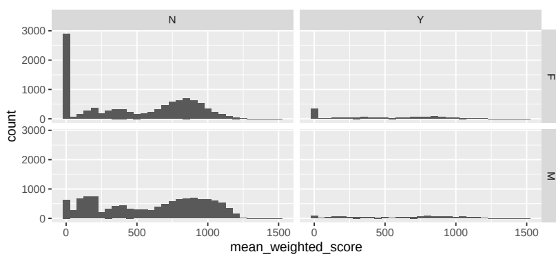
Figure 3.12. Score distributions by gender and disability status
