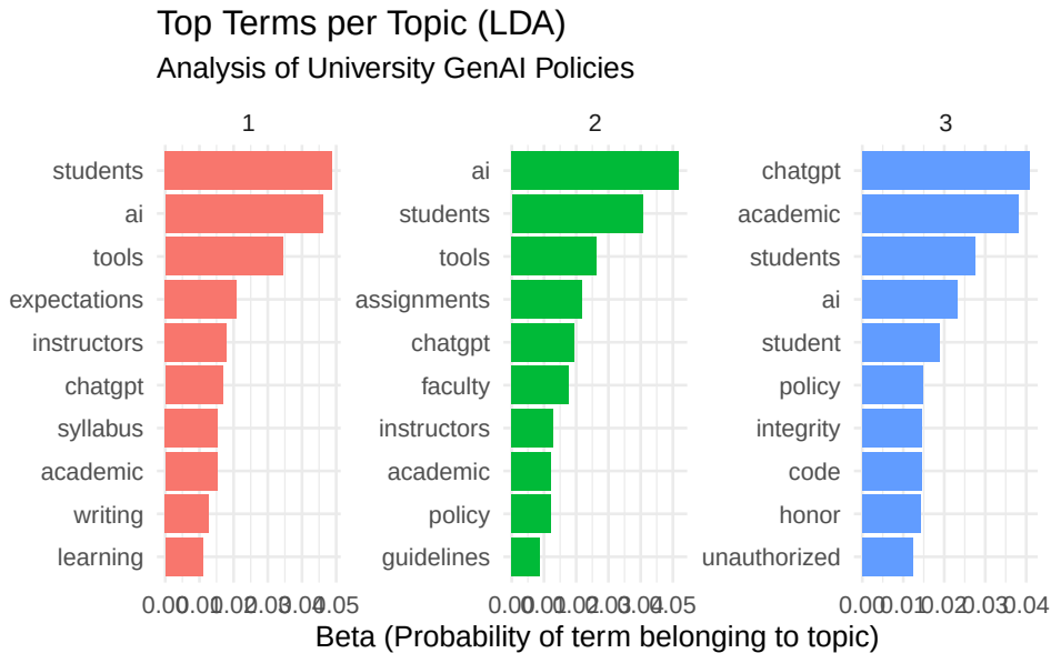
Figure 4.4. Top terms associated with the three-topic LDA model of university generative AI policies
