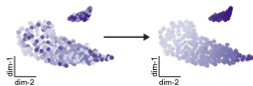
Data Denoising
