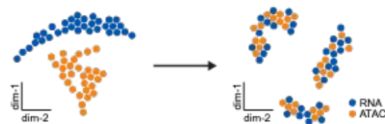
Multimodal Integration
