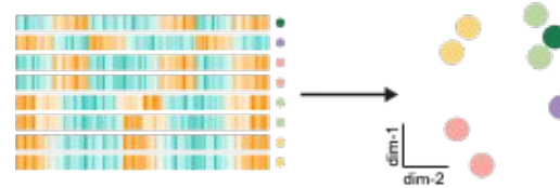
Dimensionality Reduction
