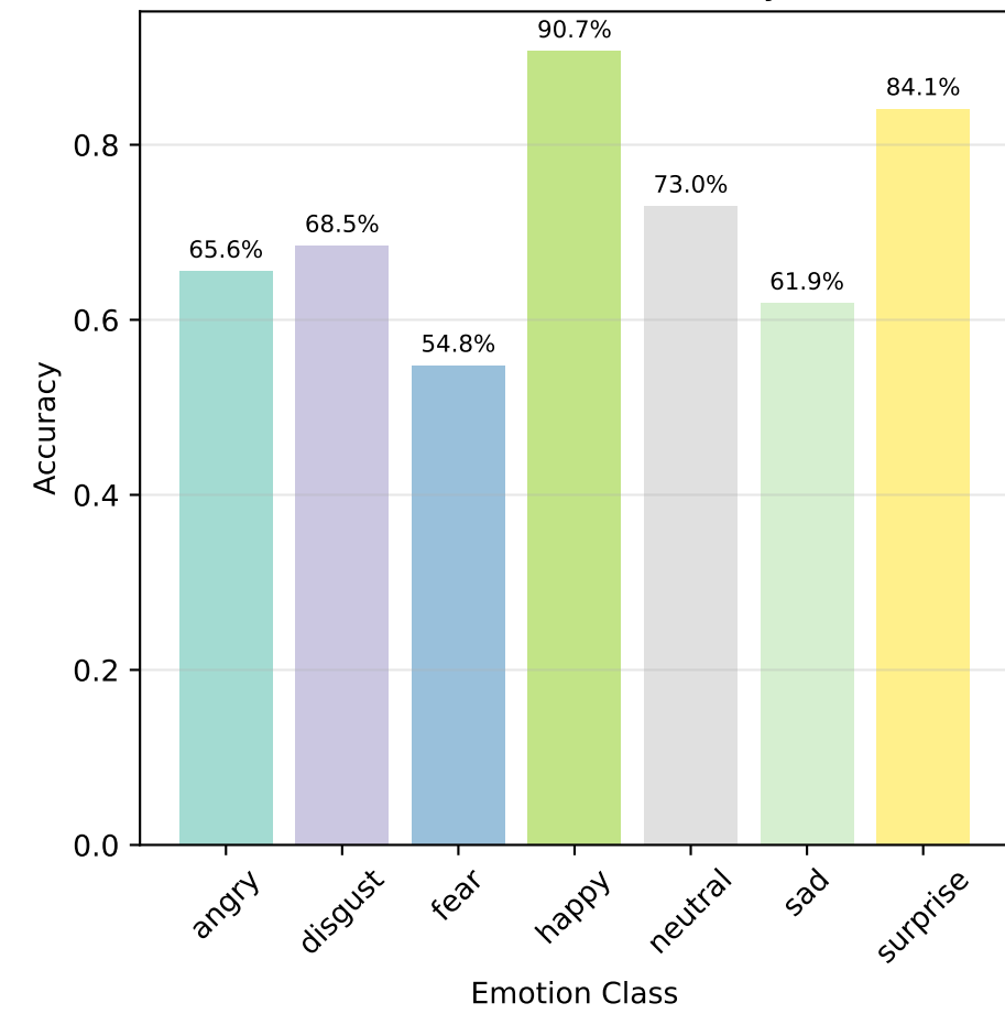
Final Per-class Accuracy
