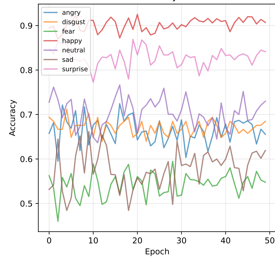
Final Per-class Accuracy
