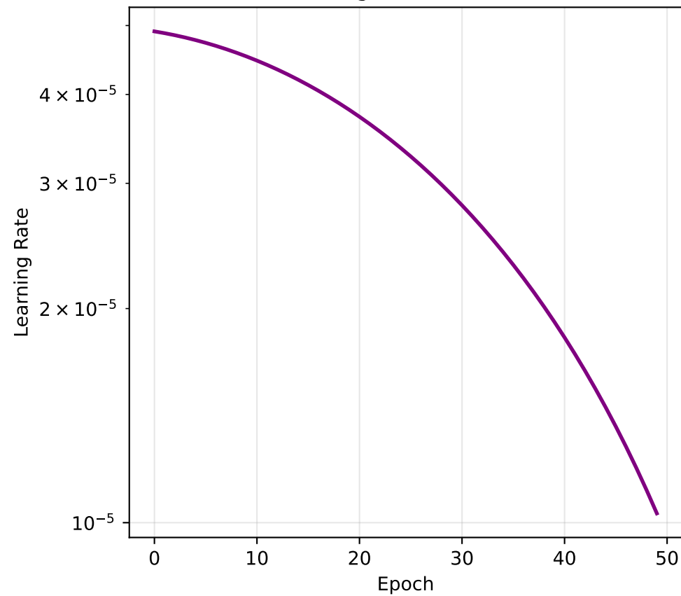
Learning Rate Schedule
