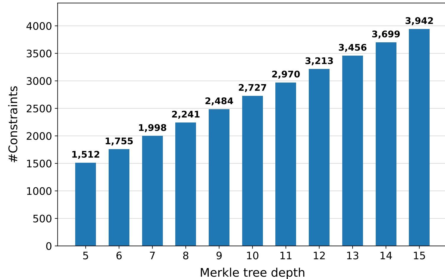
Groth16 (R1CS constraints)
