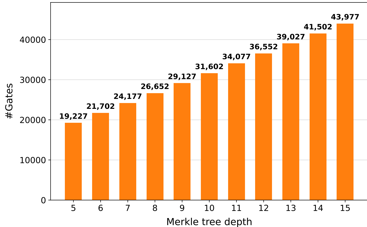
PLONK (expanded gates)
