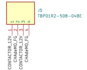
CONTACTOR +12V CONNECTOR
