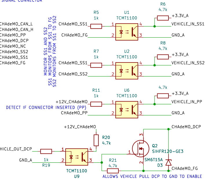
TERMINAL BLOCK TO CHAdemo SIGNAL CONNECTOR
