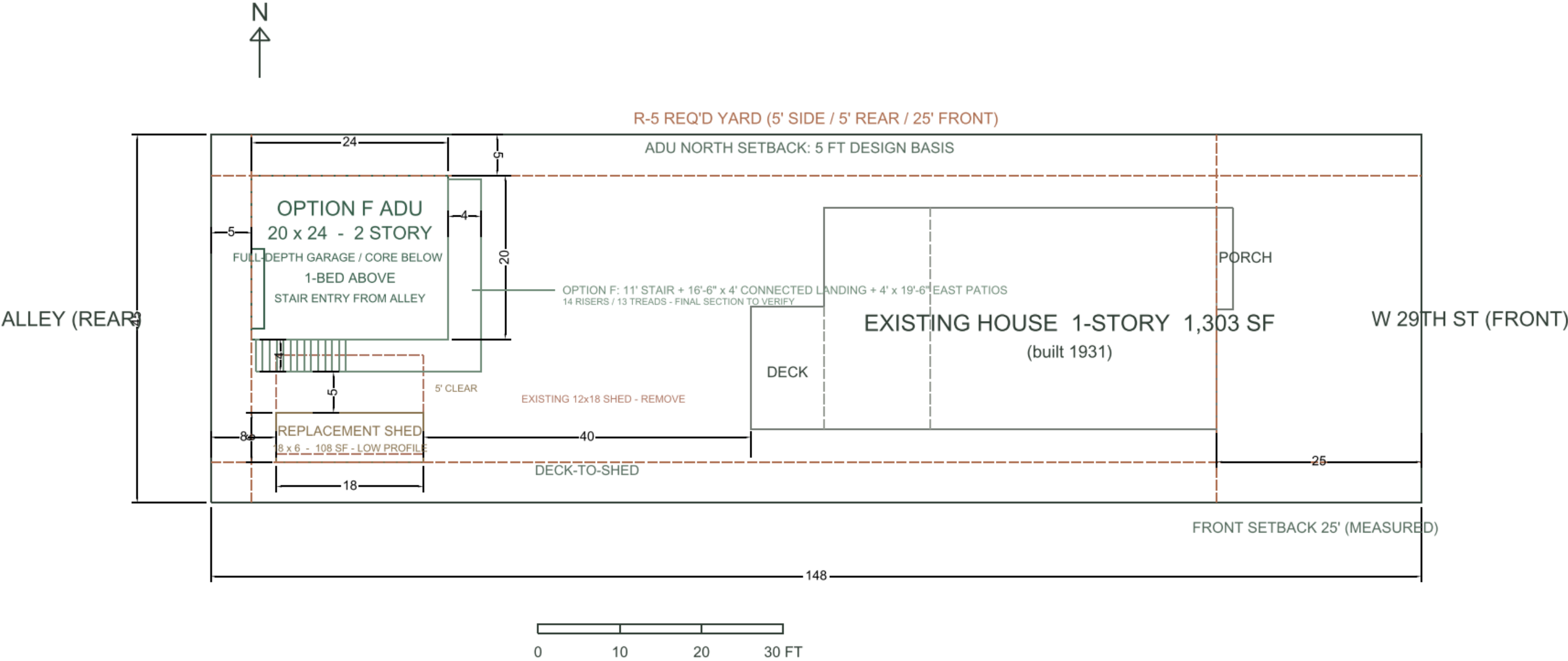
ADU SITE PLAN - 112 W 29TH ST, RICHMOND VA 23225 PIN S0001130005 - ZONE R-5 - LOT 45' x 148' (6,660 SF) - 1 UNIT = 1 FOOT - 2026-09-30 PRELIMINARY - NOT FOR CONSTRUCTION - DIMENSIONS APPROX, FIELD-VERIFY
