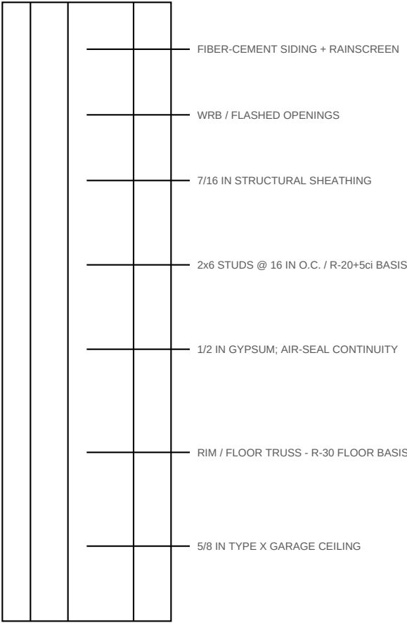
TYPICAL WALL / FLOOR EDGE - NTS
