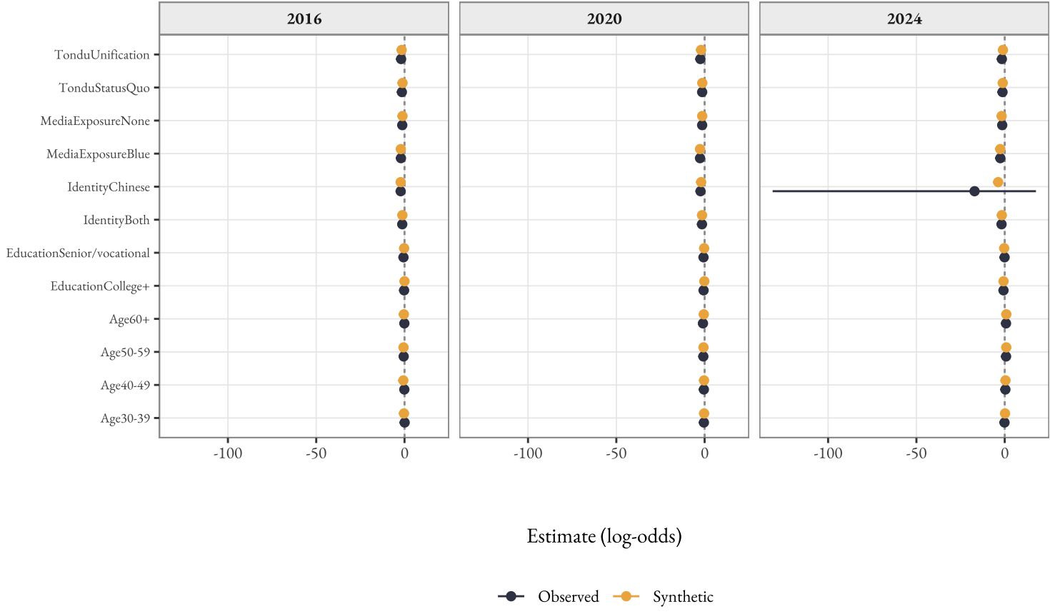
DPP vote model: observed vs synthetic
