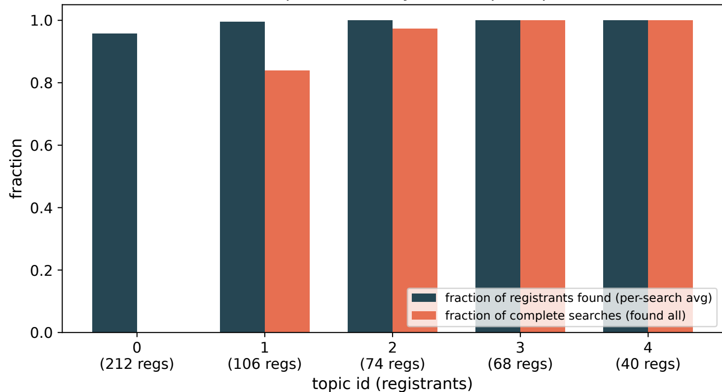
500-5topics: discovery success per topic
