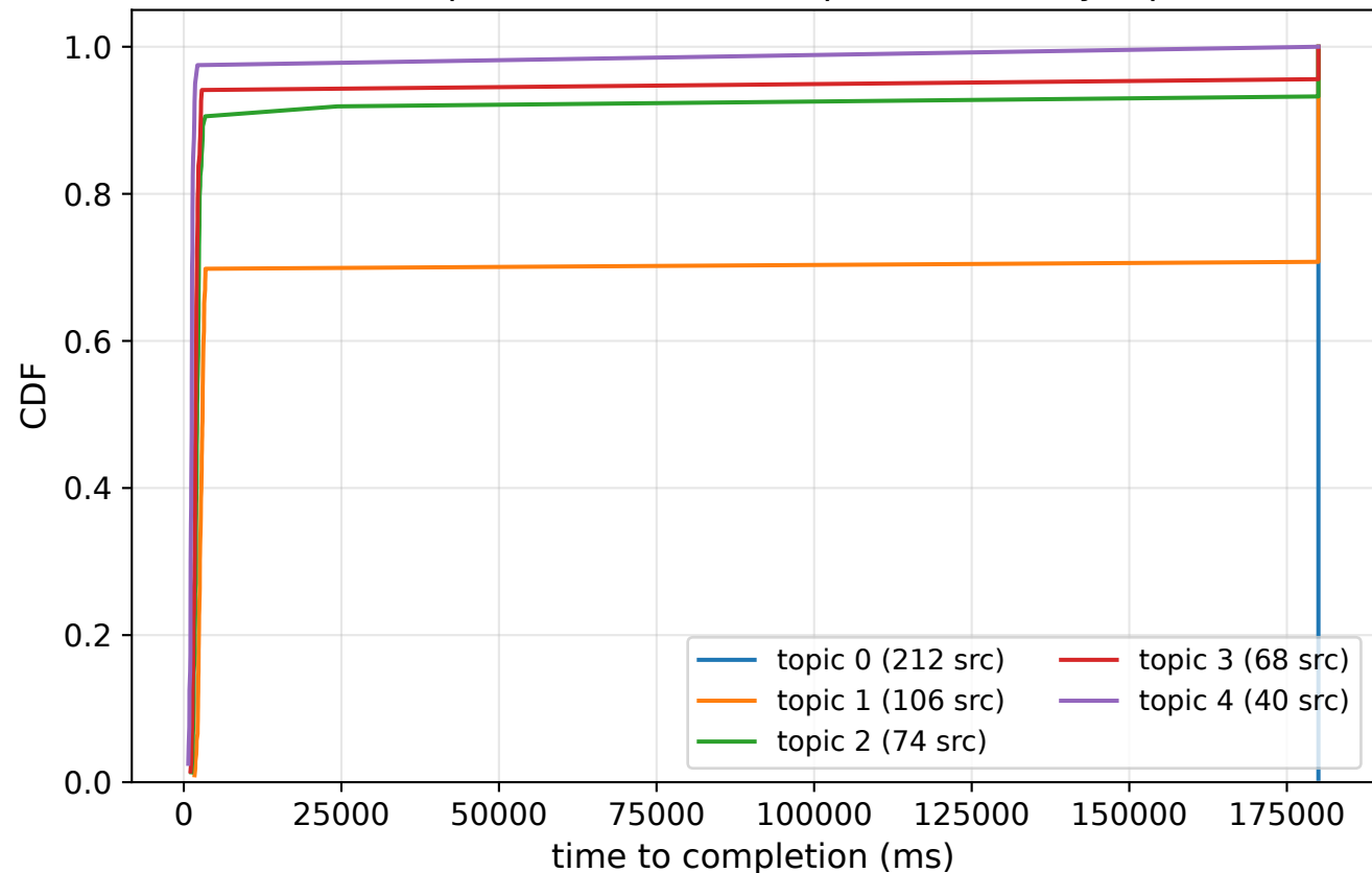
500-5topics-2x: time-to-completion CDF, by topic
