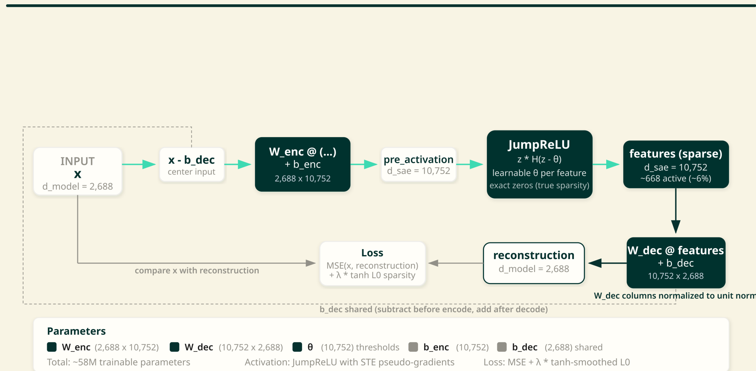
Figure 3. An overcomplete dictionary that decomposes hidden states into monosemantic features. JumpReLU thresholds \theta_i produce exact zeros (true sparsity), trained with a smooth tanh surrogate [2].
