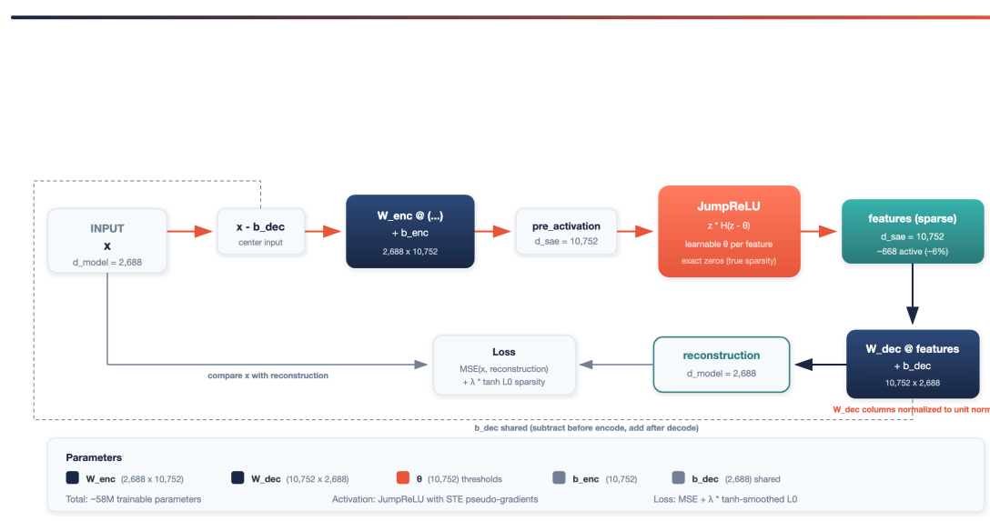
Figure 3. An overcomplete dictionary that decomposes hidden states into monosemantic features. JumpReLU thresholds \theta , produce exact zeros (true sparsity), trained with a smooth tanh surrogate [2].
