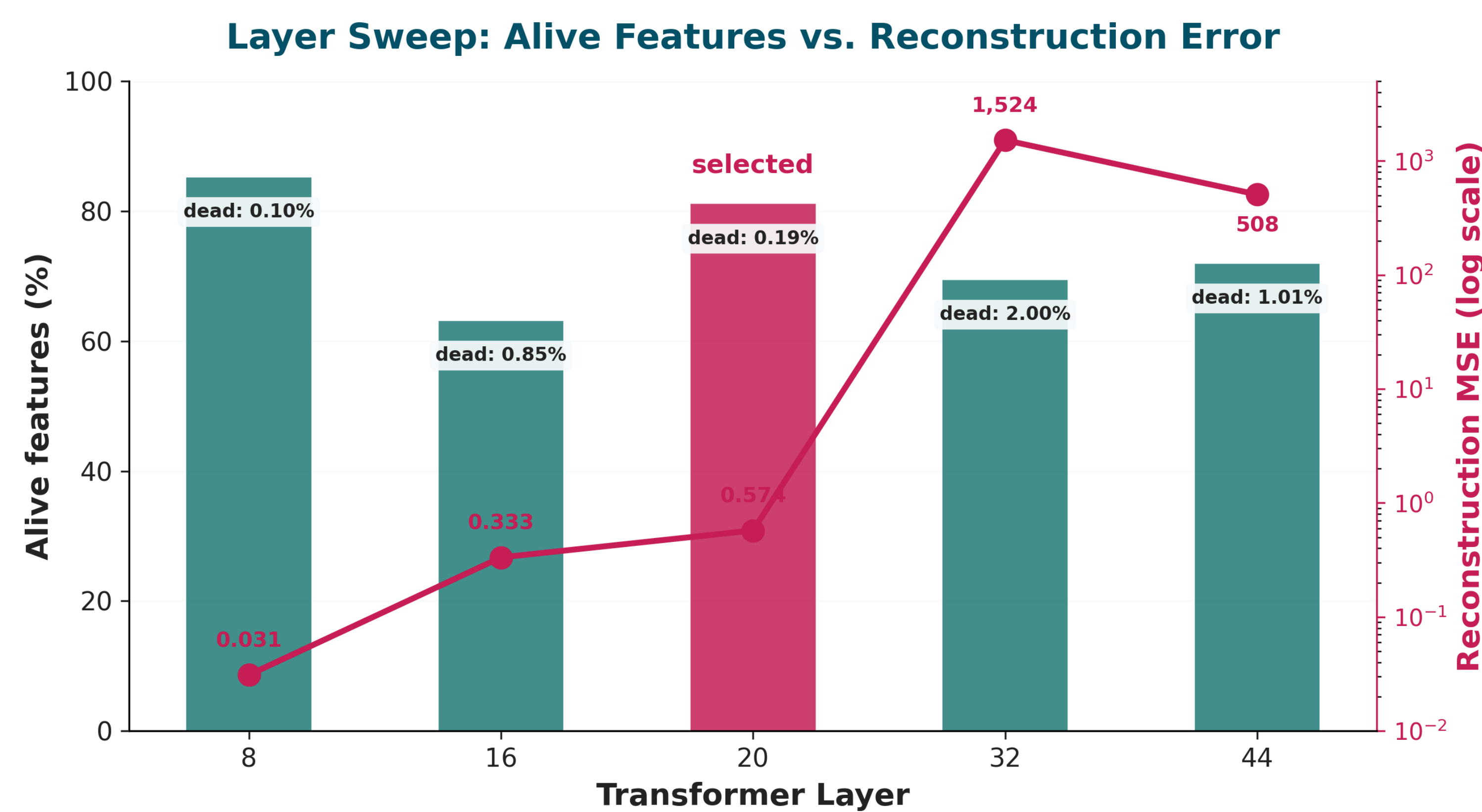
Figure 2. A single SAE cannot decompose MoE layers. Reconstruction MSE explodes by >500\times at layers 32 and 44 (sparse expert routing); layer 20 sits just before the MoE stack and gives 81.2 % alive features. Don't probe MoE layers with one SAE.
