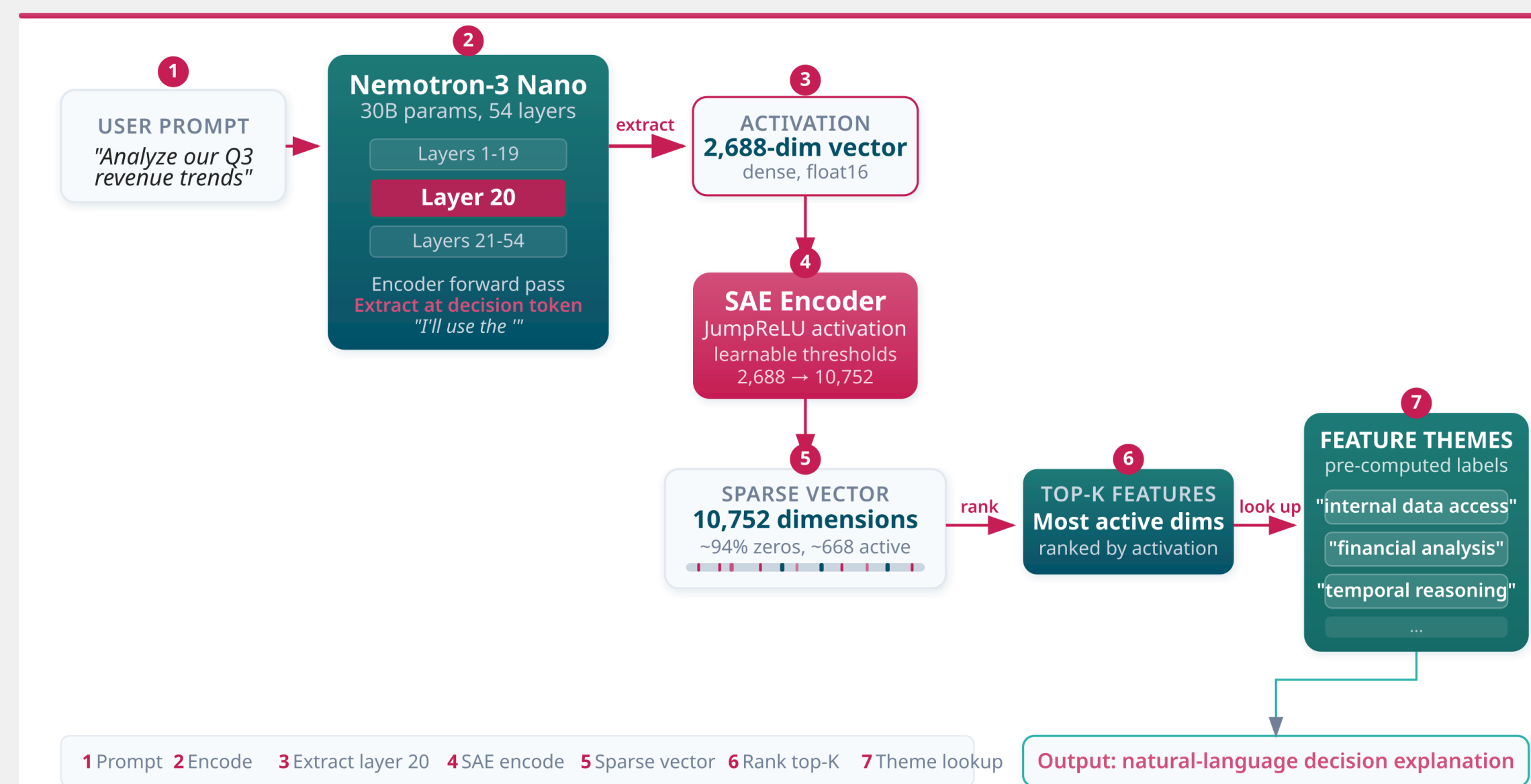
Figure 4. Every tool call ships with a rationale. At inference, the top- K active features at the decision token map to pre-computed labels — a human-readable explanation alongside the tool choice, with no extra LLM call.
