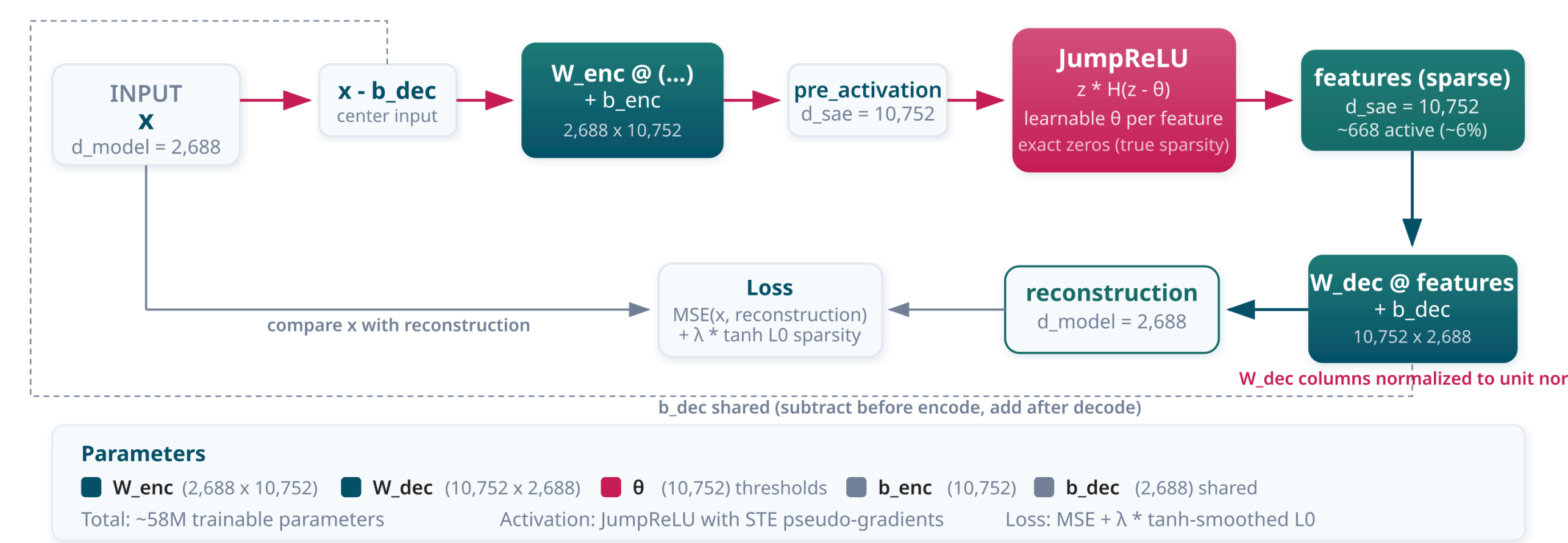
Figure 3. An overcomplete dictionary that decomposes hidden states into monosemantic features. JumpReLU thresholds \theta_i produce exact zeros (true sparsity), trained with a smooth \tanh surrogate [2].
