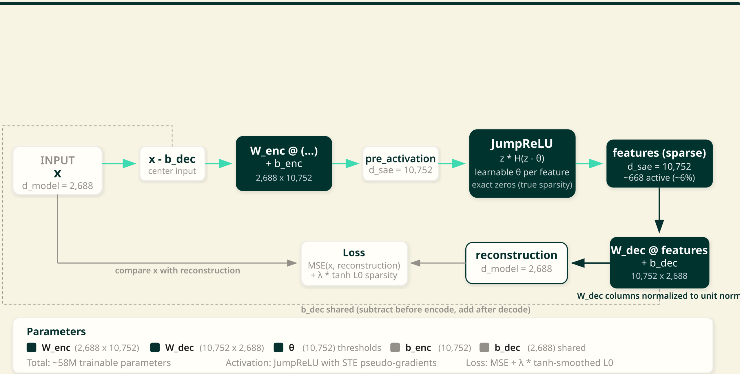
Figure 3. An overcomplete dictionary that decomposes hidden states into monosemantic features. JumpReLU thresholds \theta , produce exact zeros (true sparsity), trained with a smooth \tanh surrogate [2].
