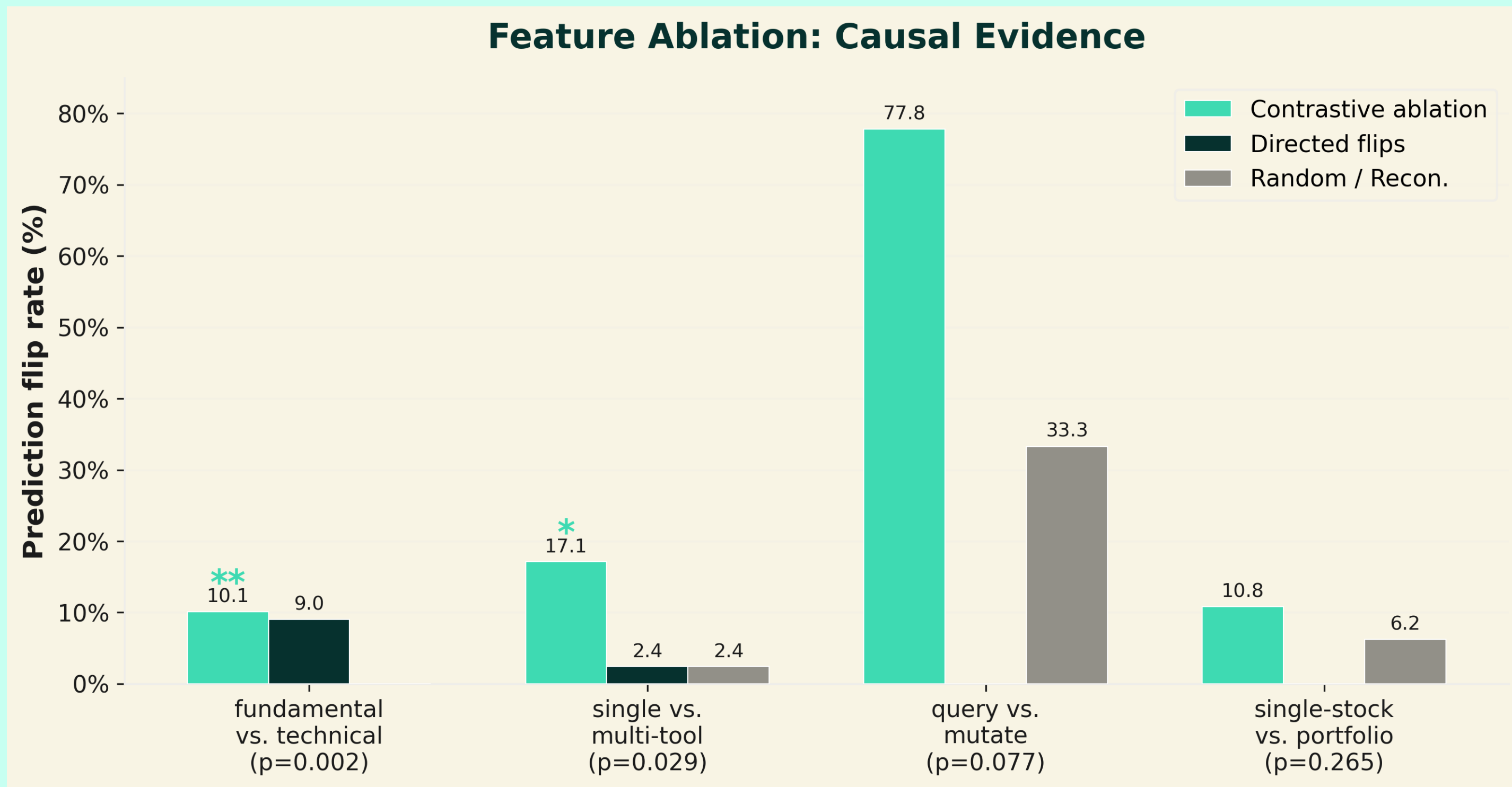
Figure 6. Ablating SAE features changes tool decisions — random features do not. Top-10 contrastive features vs. random features vs. SAE round-trip baseline.
