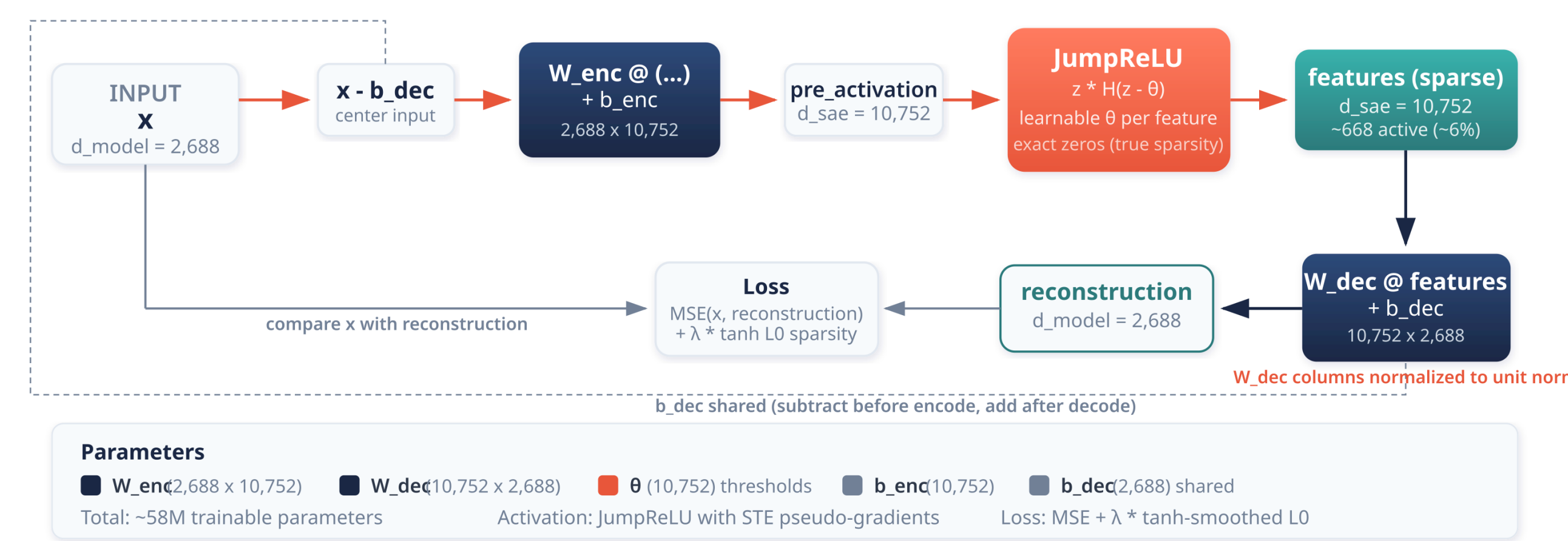
Figure 3. An overcomplete dictionary that decomposes hidden states into monosemantic features. JumpReLU thresholds \theta , produce exact zeros (true sparsity), trained with a smooth \tanh surrogate [2].
