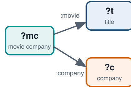
(c) Simplified query graph
