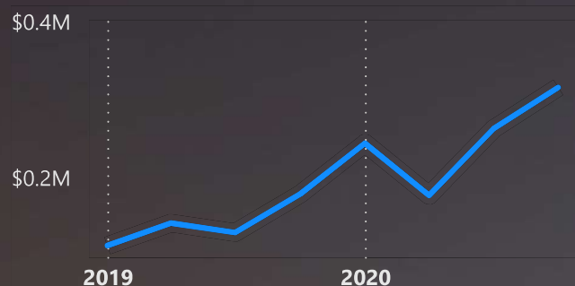
Revenue Trend
