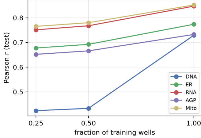
Figure 6: Test Pearson r per channel vs. the fraction of training wells (1,500-step budget).
