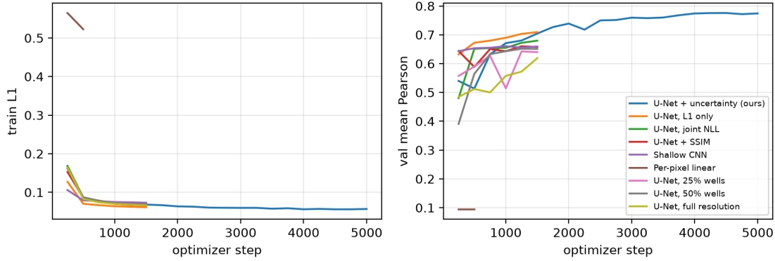
Figure 7: Training curves (train L1 and validation mean Pearson r ) of all HepatoPAC experiments.
