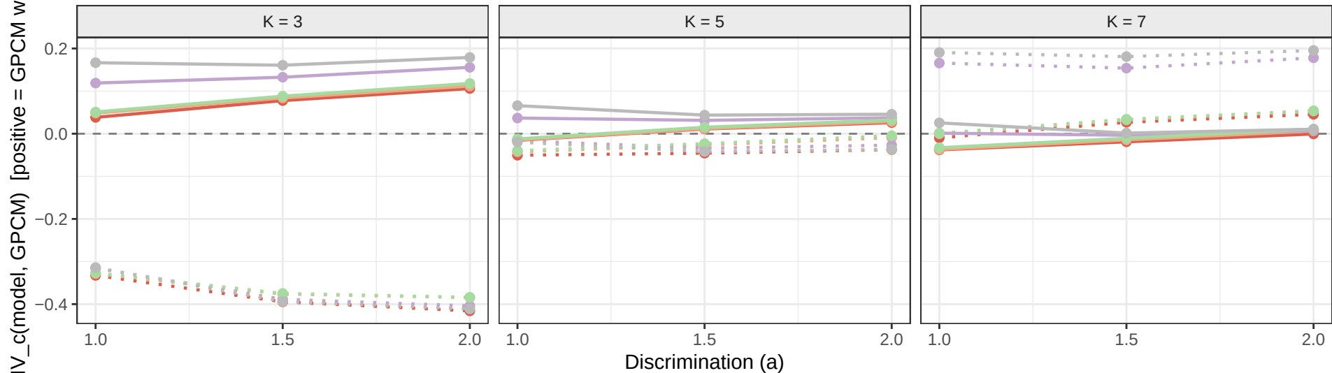
Binomial approximations: symmetric vs. asymmetric thresholds
