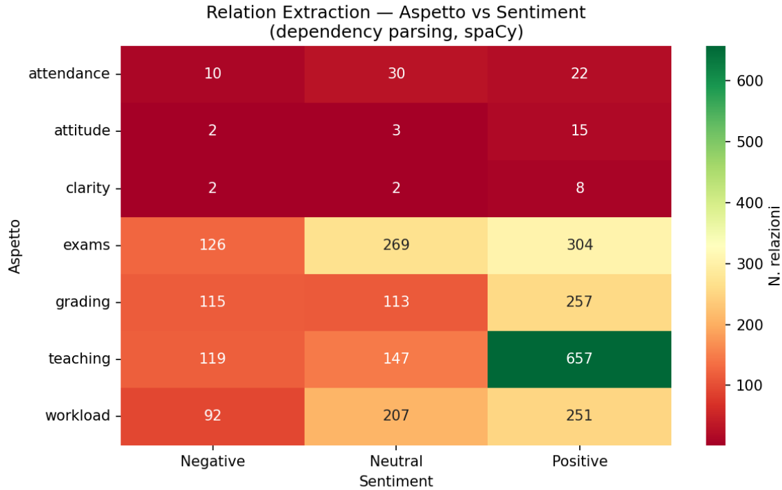
Figura 16: Heatmap aspetto \times sentiment (relation extraction, dependency parsing)
