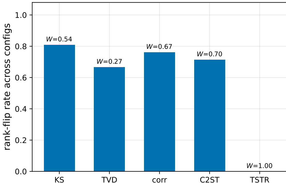
Ranking instability by metric (diabetes, 15 seeds)
